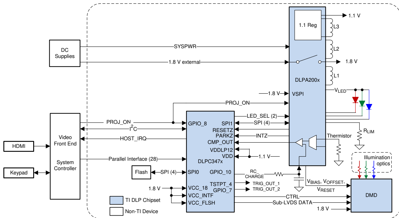
图 8-1. Typical Application
