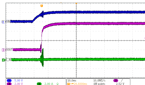
图 7-4. DCP020505P Start-Up at 10% Load
