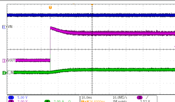
图 7-6. DCP020505P Enable Start-Up at 100% Load
