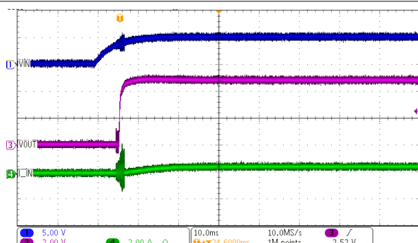
图 7-5. DCP020505P Start-Up at 100% Load
