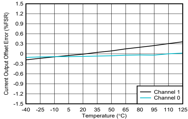
图 6-45. Current Output Offset Error vs Temperature
