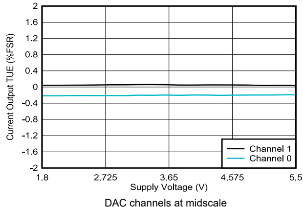
图 6-44. Current Output TUE vs Supply Voltage
