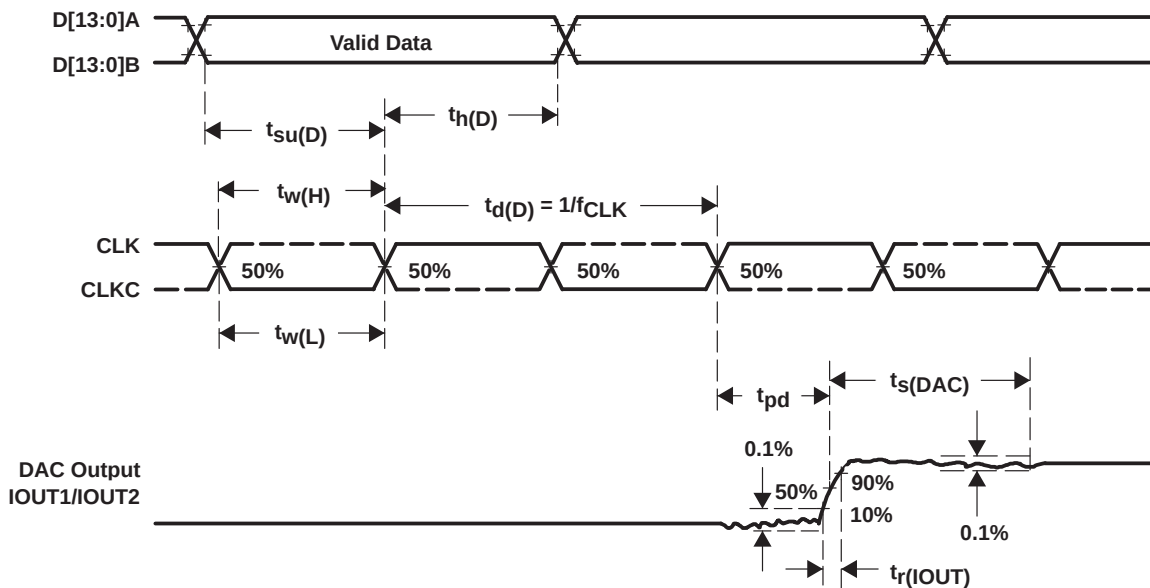
Figure 5. Timing Diagram
