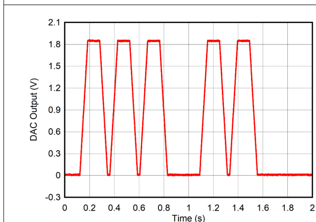
图 9-10. High-Priority Alarm
