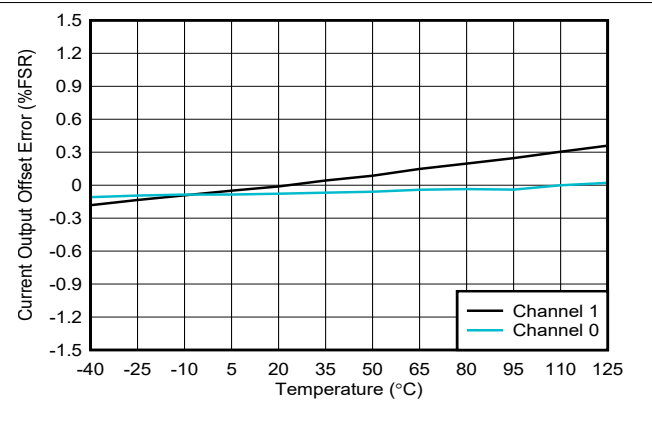
图 6-45. Current Output Offset Error vs Temperature
