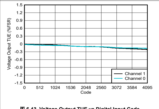
图 6-13. Voltage Output TUE vs Digital Input Code
