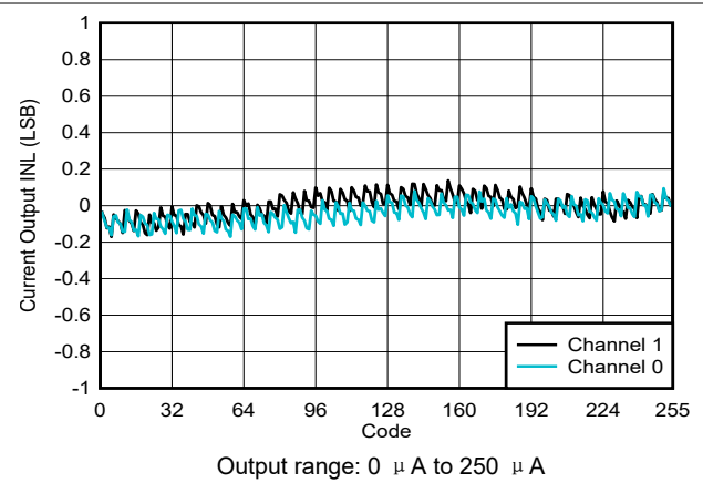
图 6-31. Current Output INL vs Digital Input Code
