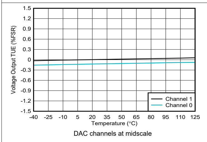
图 6-14. Voltage Output TUE vs Temperature
