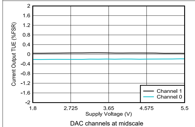
图 6-44. Current Output TUE vs Supply Voltage
