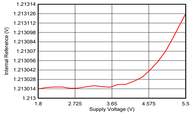
图 6-61. Internal Reference vs Supply Voltage
