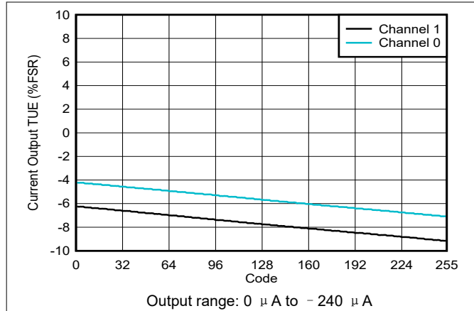
图 6-42. Current Output TUE vs Digital Input Code
