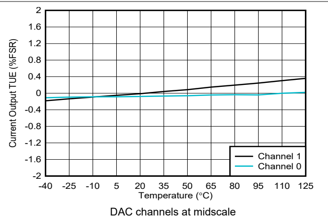
图 6-43. Current Output TUE vs Temperature
