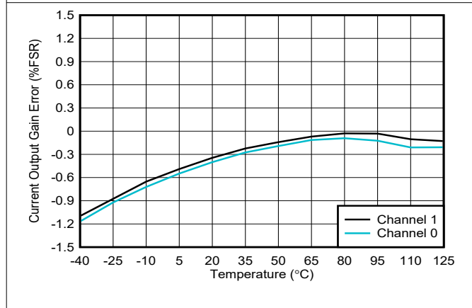
图 6-46. Current Output Gain Error vs Temperature
