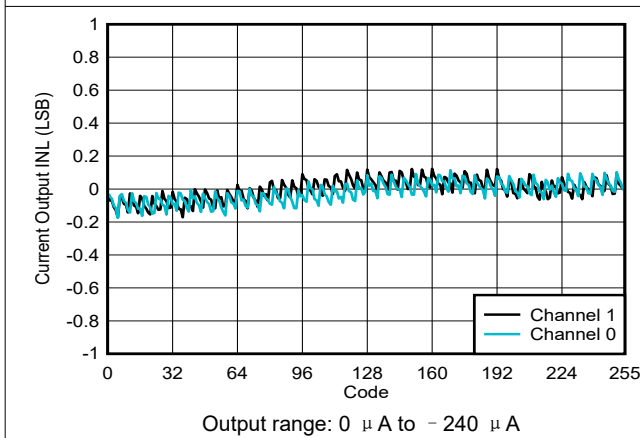
图 6-32. Current Output INL vs Digital Input Code
