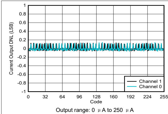
图 6-36. Current Output DNL vs Digital Input Code
