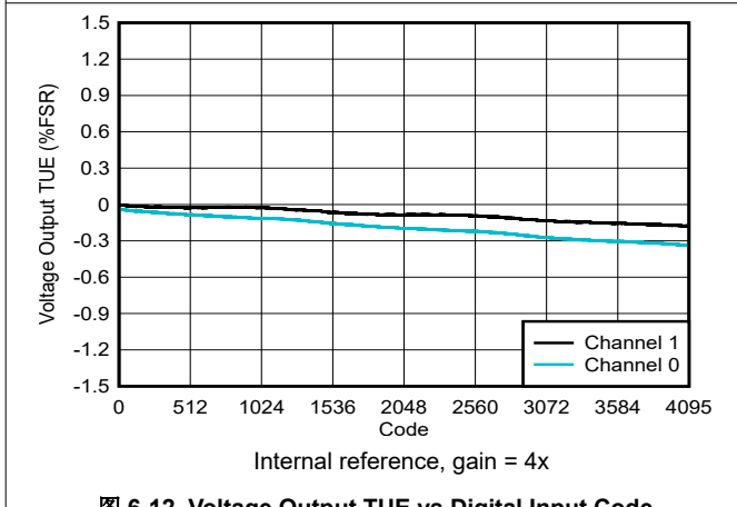
图 6-12. Voltage Output TUE vs Digital Input Code
