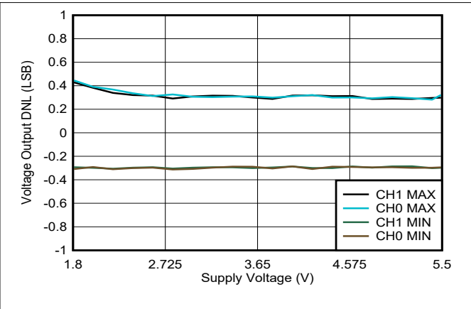
图 6-11. Voltage Output DNL vs Supply Voltage
