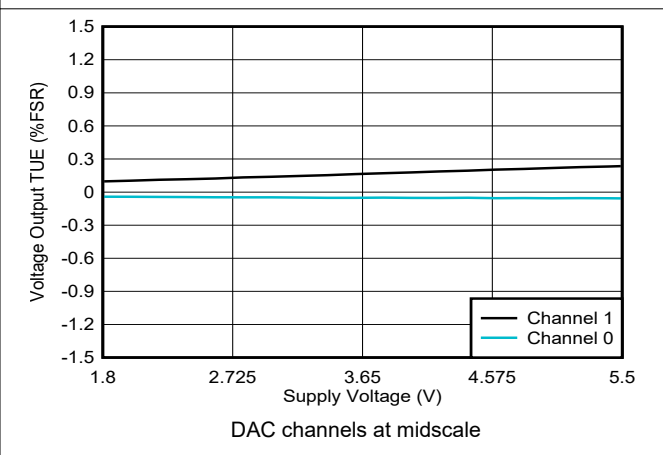
图 6-15. Voltage Output TUE vs Supply Voltage
