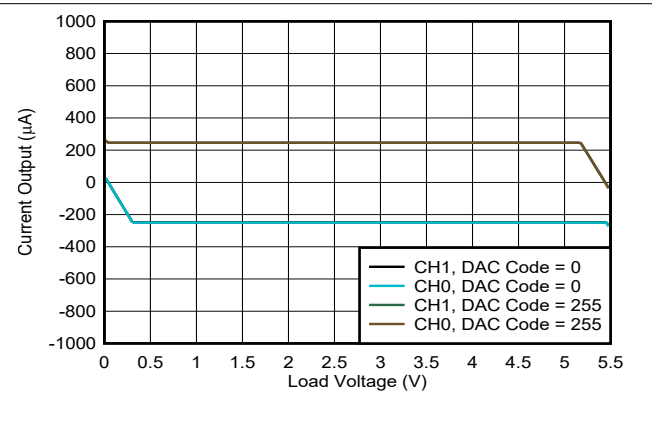
图 6-47. Current Output vs Load Voltage
