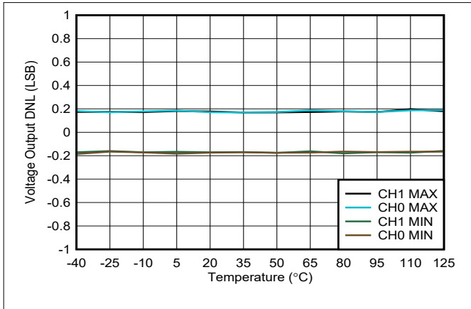
图 6-10. Voltage Output DNL vs Temperature
