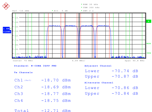
Figure 40. DAC3164 ACPR Four-Carrier WCDMA Test Mode 1
