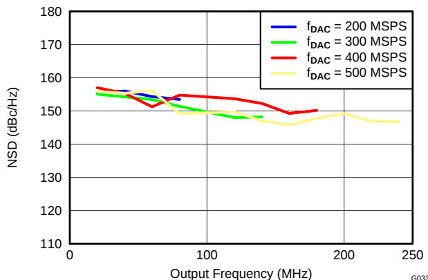
Figure 33. DAC3164 NSD vs Output Frequency Over f_{DAC}
