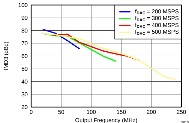
Figure 10. DAC3154 IMD3 vs Output Frequency Over f_{DAC}
