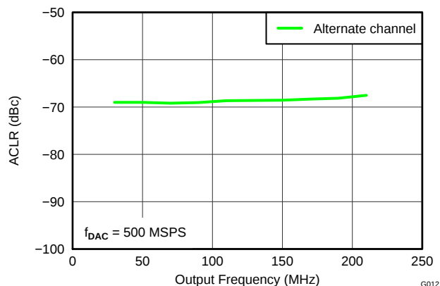
Figure 14. DAC3154 ACLR (Alternate Channel) vs Output Frequency
