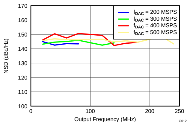
Figure 12. DAC3154 NSD vs Output Frequency Over f_{DAC}
