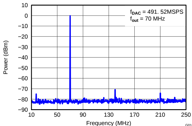
Figure 16. DAC3154 Single-Tone Spectral Plot (IF = 70MHz)
