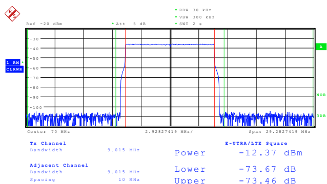
Figure 42. DAC3164 ACPR LTE 10-MHz FDD E-TM 1.1
