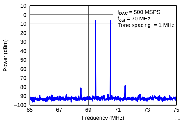
Figure 18. DAC3154 Two-Tone Spectral Plot (IF = 70MHz)
