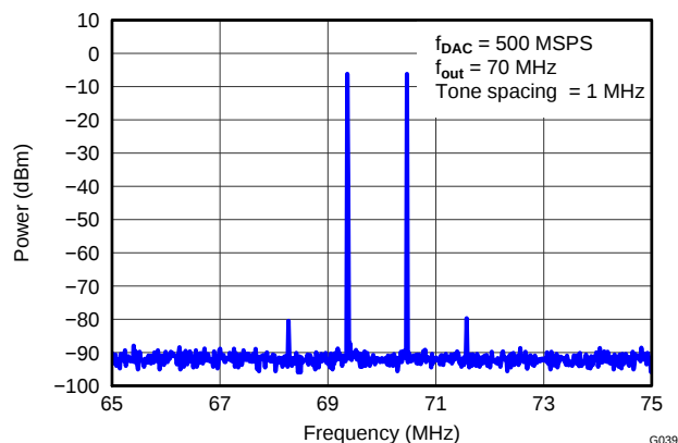
Figure 39. DAC3164 Two-Tone Spectral Plot (IF = 70MHz)
