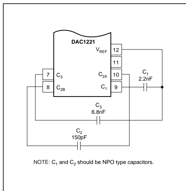
FIGURE 1. Capacitor Connections.
