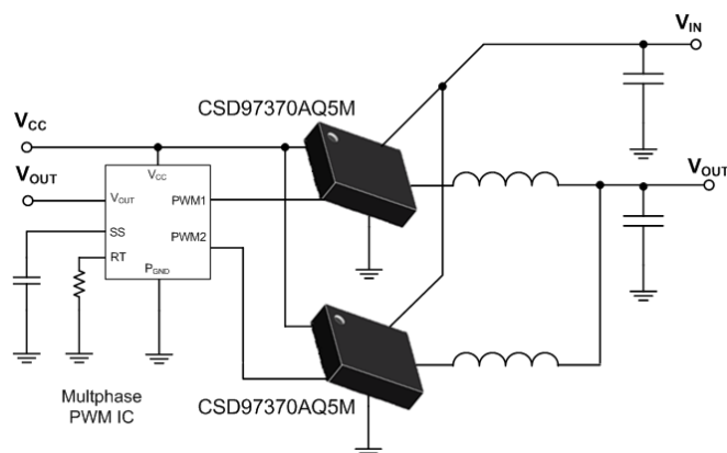
Figure 1. Application Diagram
