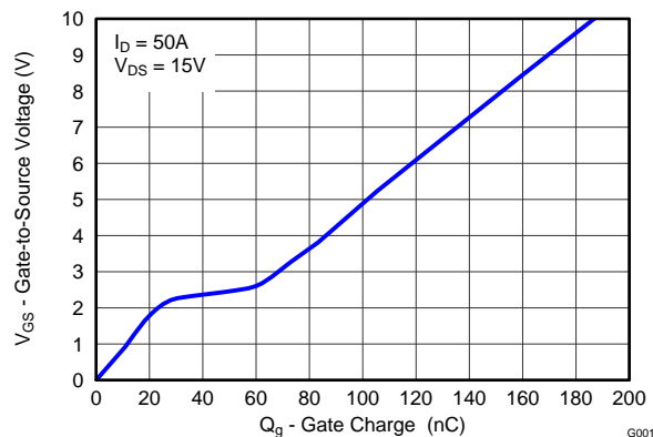
栅极电荷
