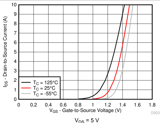
图 5-2. Transfer Characteristics
