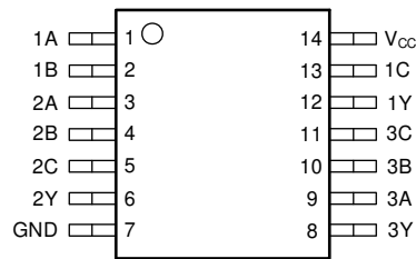
图 5-1. D, N, or J Package 14-Pin SOIC, PDIP, or CDIP Top View
