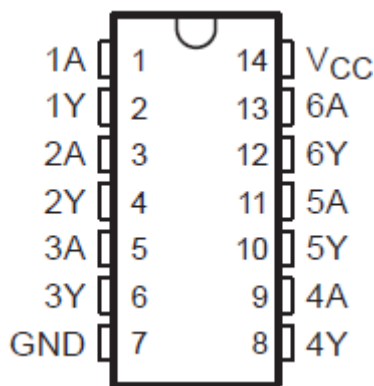
图 3-1. CD54AC04 J Package, 14-Pin CDIP; CD74AC04 N or D Package, 14-Pin SOIC or PDIP (Top View)
