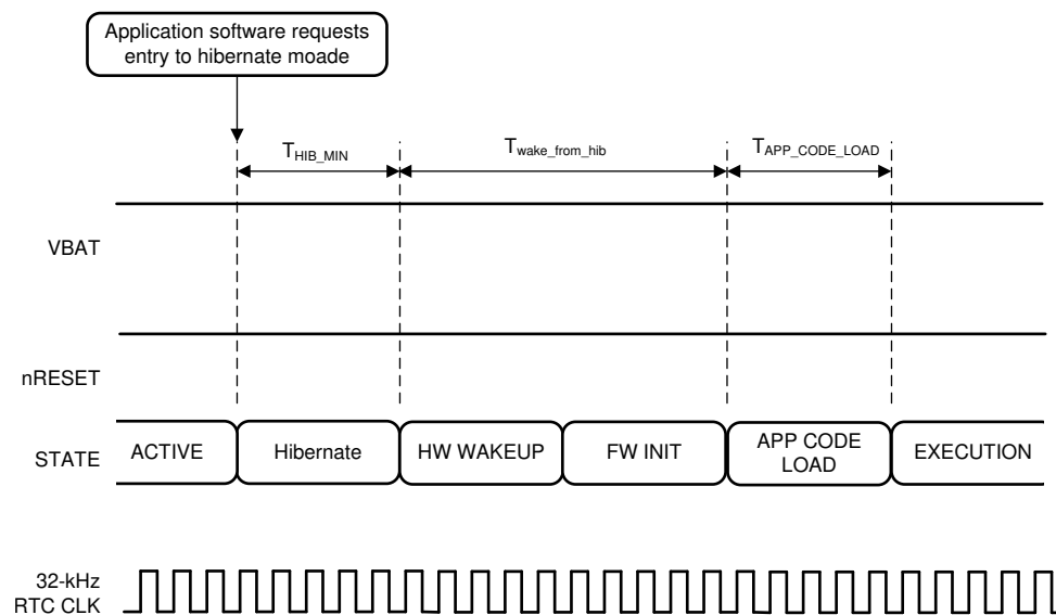
图 7-8. Wakeup From HIBERNATE Timing Diagram
