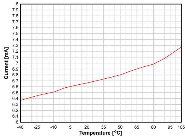
图 8-7. RX Current versus Temperature (WBMS, 2.44 GHz)
