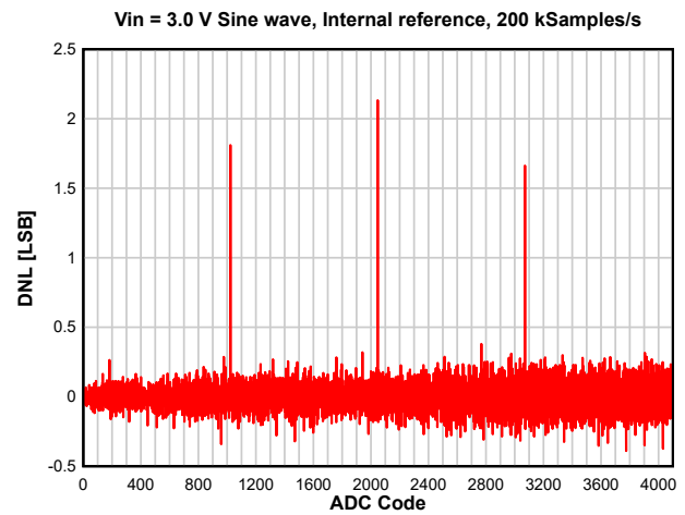
图 8-24. DNL versus ADC Code
