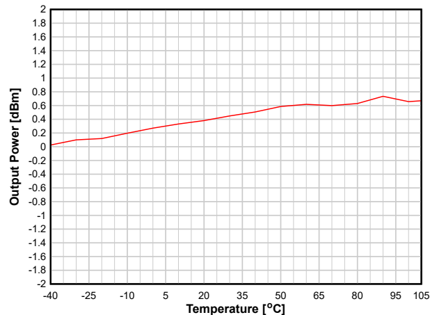
图 8-15. Output Power vs. Temperature (WBMS, 2.44 GHz, 0dBm)
