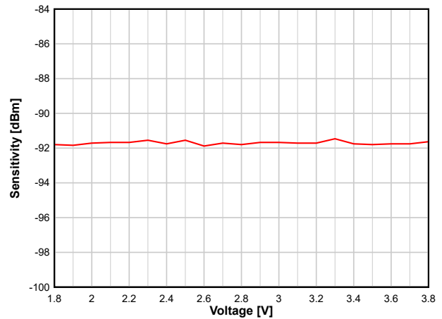
图 8-14. Sensitivity versus Supply Voltage (VDDS) (WBMS, 2.44 GHz, DCDC off)
