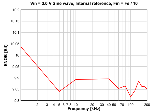
图 8-22. ENOB versus Sampling Frequency
