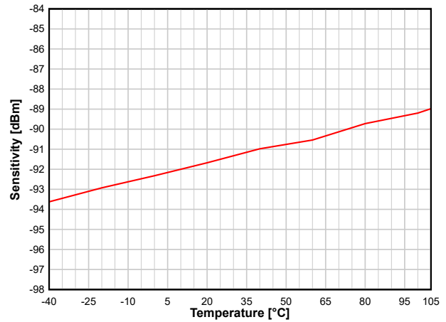
图 8-12. Sensitivity versus Temperature (WBMS, 2.44 GHz)
