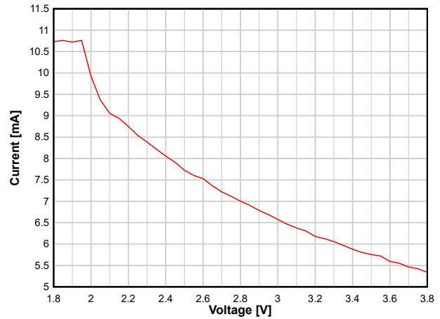
图 8-8. RX Current versus Supply Voltage (VDDSD) (WBMS, 2.44 GHz)
