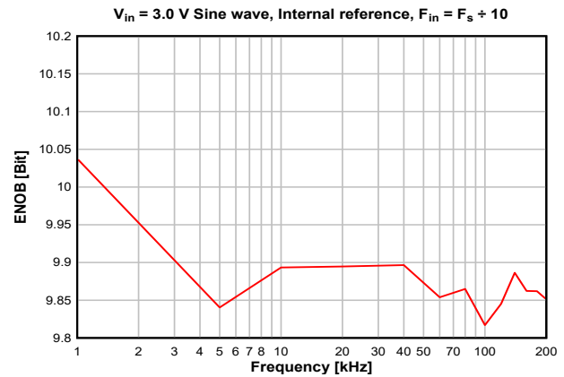
图 8-24. ENOB vs. Sampling Frequency
