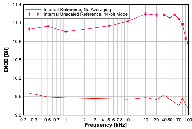
图 8-23. ENOB vs. Input Frequency
