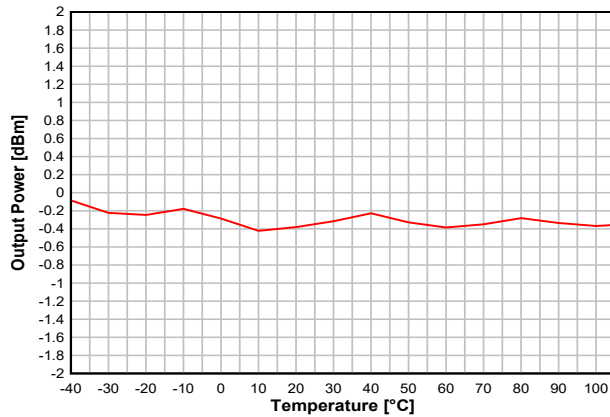
图 8-17. Output Power vs. Temperature (BLE 1 Mbps, 2.44 GHz, 0 dBm)
