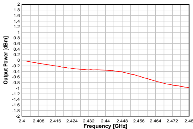
图 8-21. Output Power vs. Frequency (BLE 1 Mbps, 2.44 GHz, 0 dBm)
