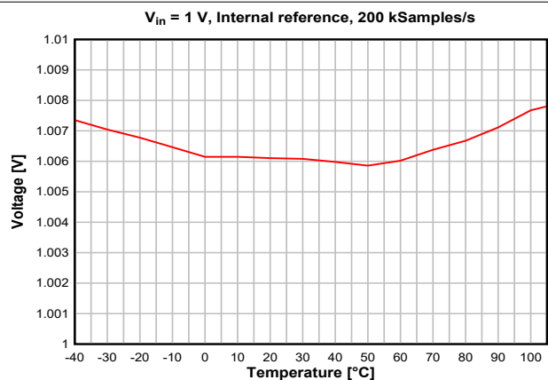
图 8-27. ADC Accuracy vs. Temperature
