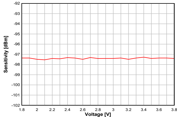
图 8-14. Sensitivity vs. Supply Voltage (VDD) (BLE 1 Mbps, 2.44 GHz)
