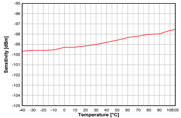
图 8-13. Sensitivity vs. Temperature (IEEE 802.15.4-2006, 250 kbps, OQPSK DSSS 1:8, 2.44 GHz)
