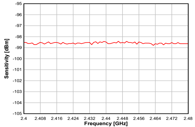
图 8-11. Sensitivity vs. Frequency (IEEE 802.15.4-2006, 250 kbps, OQPSK DSSS 1:8, 2.44 GHz)
