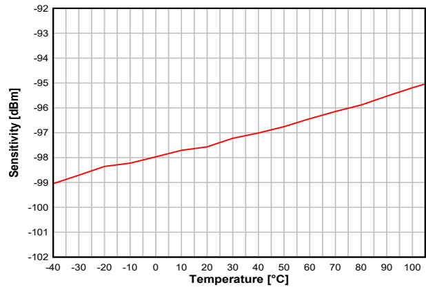
图 8-12. Sensitivity vs. Temperature (BLE 1 Mbps, 2.44 GHz)
