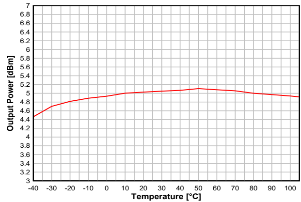
图 8-18. Output Power vs. Temperature (BLE 1 Mbps, 2.44 GHz, +5 dBm)
