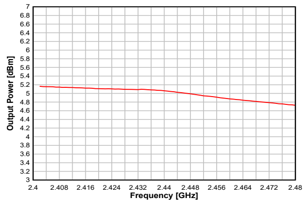
图 8-22. Output Power vs. Frequency (BLE 1 Mbps, 2.44 GHz, +5 dBm)
