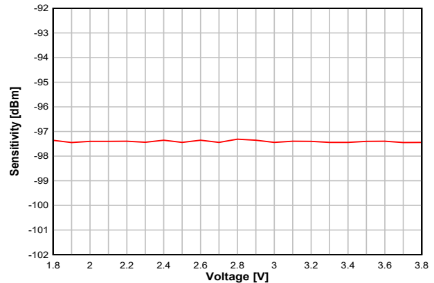
图 8-15. Sensitivity vs. Supply Voltage (VDD) (BLE 1 Mbps, 2.44 GHz, DCDC Off)
