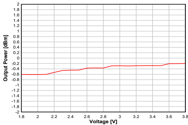
图 8-19. Output Power vs. Supply Voltage (VDD5) (BLE 1 Mbps, 2.44 GHz, 0 dBm)
