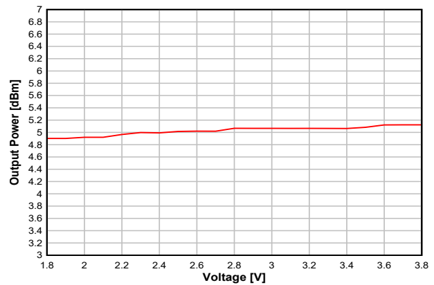
图 8-20. Output Power vs. Supply Voltage (VDD5) (BLE 1 Mbps, 2.44 GHz, +5 dBm)
