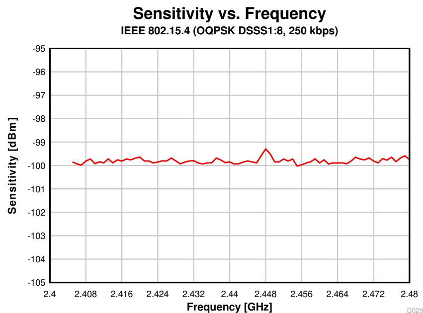
图 8-15. Sensitivity vs. Frequency (250 kbps, 2.44 GHz)
