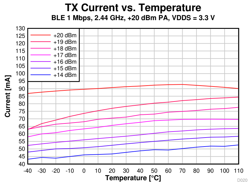
图 8-9. TX Current vs. Temperature (BLE 1 Mbps, 2.44 GHz, VDD = 3.3 V)
