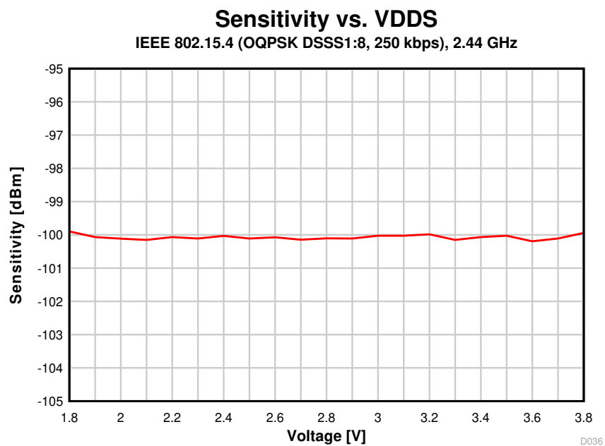
8-20. Sensitivity vs. Supply Voltage (VDD) (250 kbps, 2.44 GHz)
