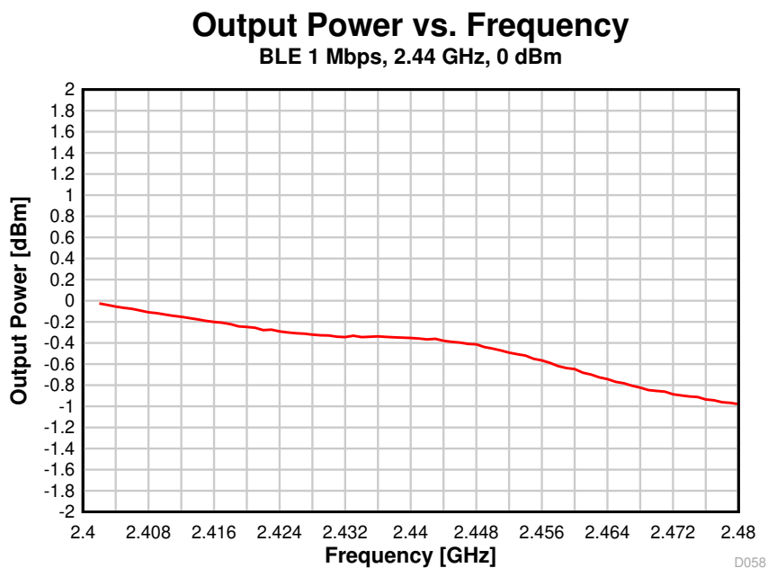
图 8-29. Output Power vs. Frequency (BLE 1 Mbps, 2.44 GHz)
