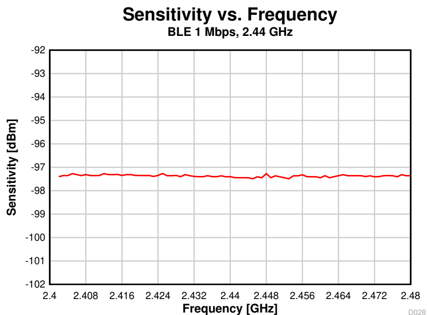
图 8-14. Sensitivity vs. Frequency (BLE 1 Mbps, 2.44 GHz)
