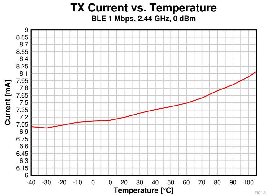
图 8-8. TX Current vs. Temperature (BLE 1 Mbps, 2.44 GHz)
