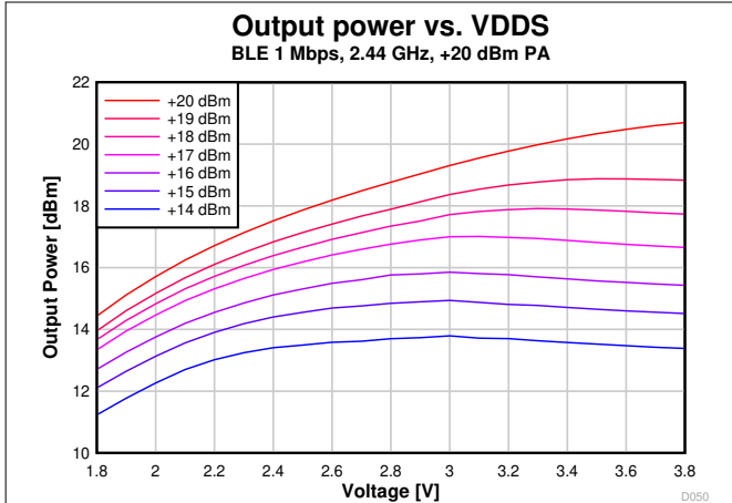
图 8-27. Output Power vs. Supply Voltage (VDD) (BLE 1 Mbps, 2.44 GHz, +20 dBm PA)
