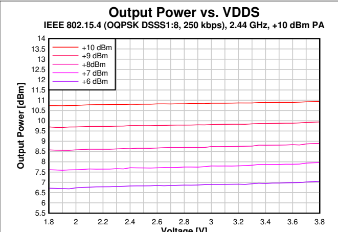
图 8-28. Output Power vs. Supply Voltage (VDD) (2.44 GHz, +10 dBm PA)
