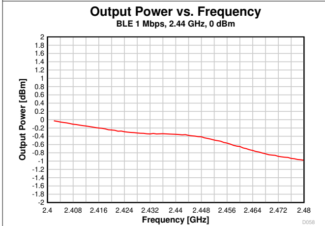
图 8-29. Output Power vs. Frequency (BLE 1 Mbps, 2.44 GHz)
