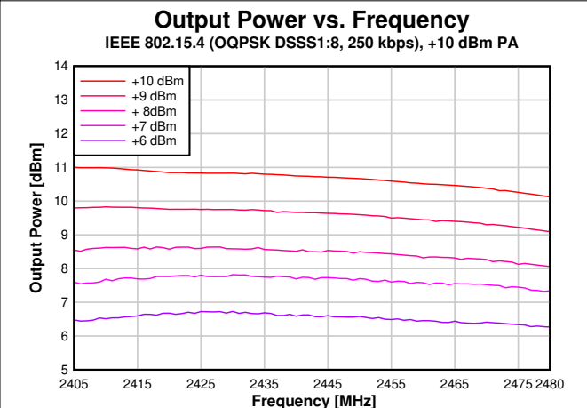
图 8-32. Output Power vs. Frequency (250 kbps, +10 dBm PA)
