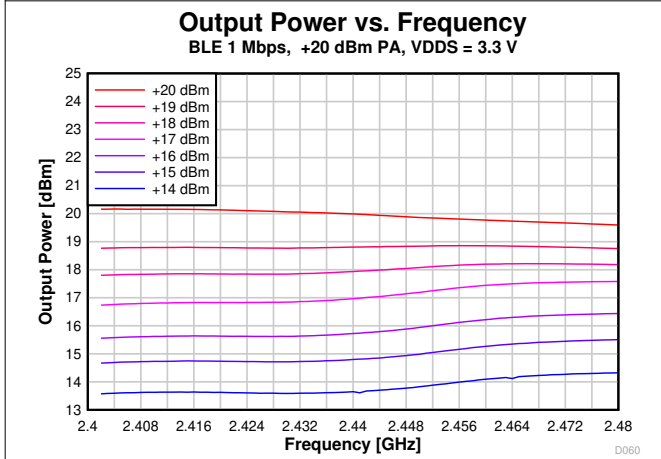
图 8-31. Output Power vs. Frequency (BLE 1 Mbps, 2.44 GHz, +20 dBm PA)
