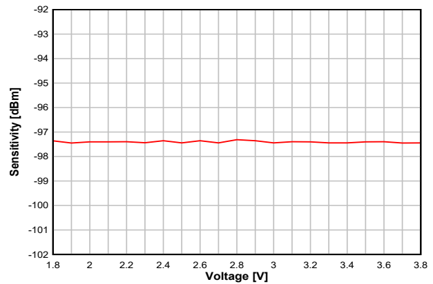
图 8-13. Sensitivity vs. Supply Voltage (VDD) (BLE 1 Mbps, 2.44 GHz, DCDC Off)
