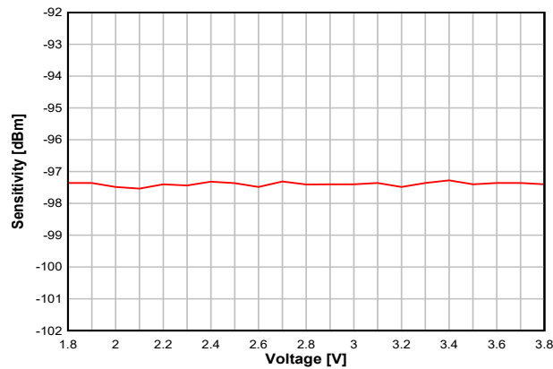
图 8-12. Sensitivity vs. Supply Voltage (VDD) (BLE 1 Mbps, 2.44 GHz)
