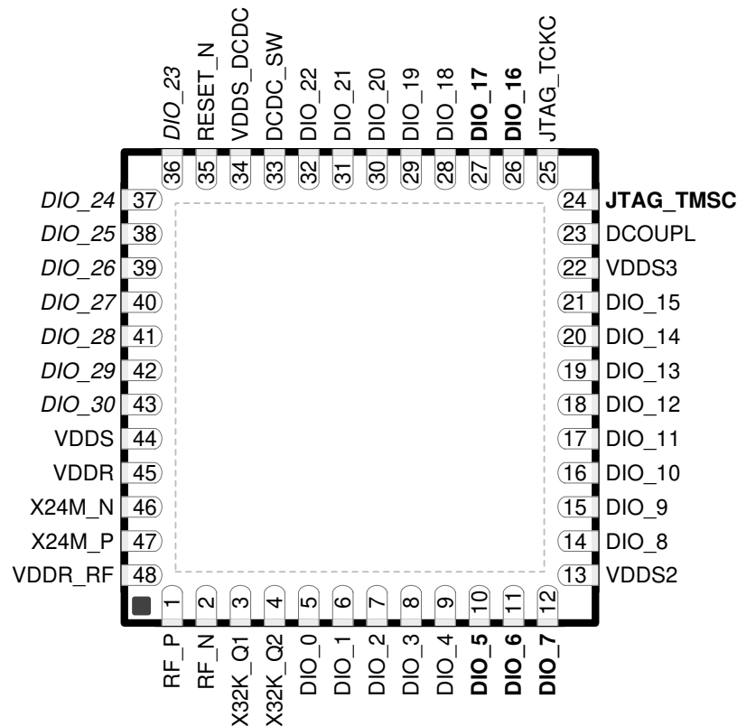
图 7-1. RGZ Package 48-Pin VQFN (7-mm x 7-mm) Pinout, 0.5-mm Pitch
