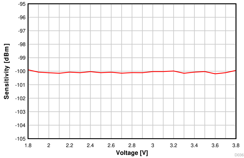
8-27. Sensitivity vs. Supply Voltage (VDD5) (250 kbps, 2.44 GHz)
