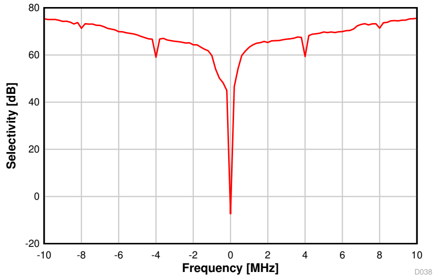
8-28. Selectivity vs. Frequency Offset (50 kbps, 868.3 MHz)
