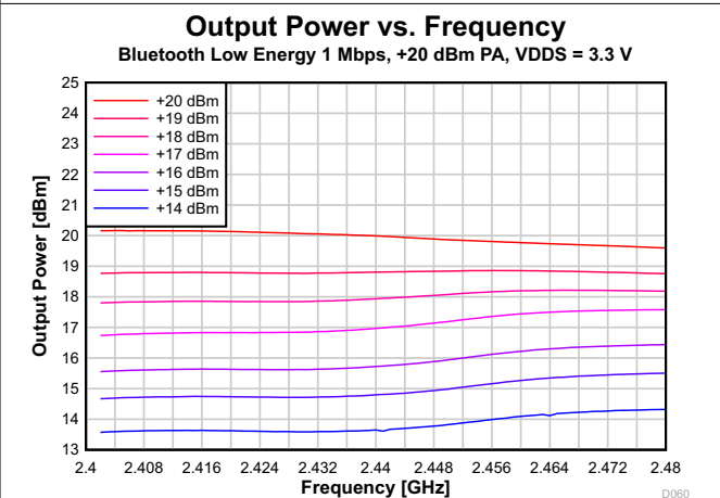
图 7-52. Output Power vs. Frequency (Bluetooth Low Energy 1 Mbps, 2.44 GHz, +20 dBm PA)
