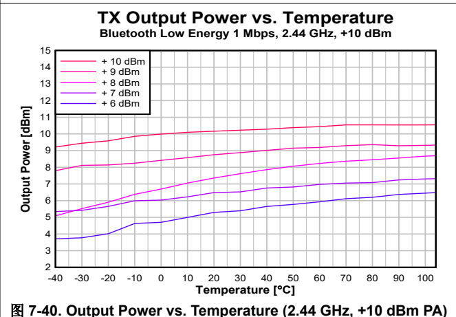
图 7-40. Output Power vs. Temperature (2.44 GHz, +10 dBm PA)
