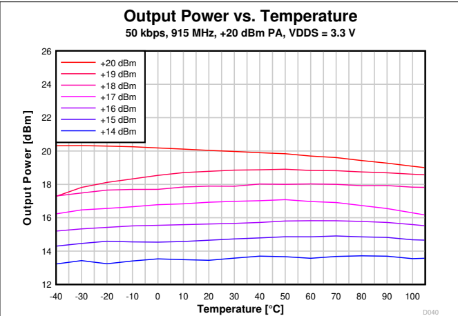
图 7-36. Output Power vs. Temperature (50 kbps, 915 MHz)
