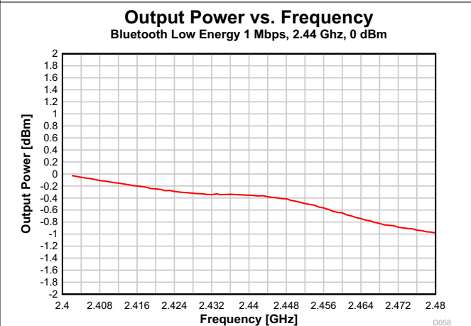
图 7-50. Output Power vs. Frequency (Bluetooth Low Energy 1 Mbps, 2.44 GHz)
