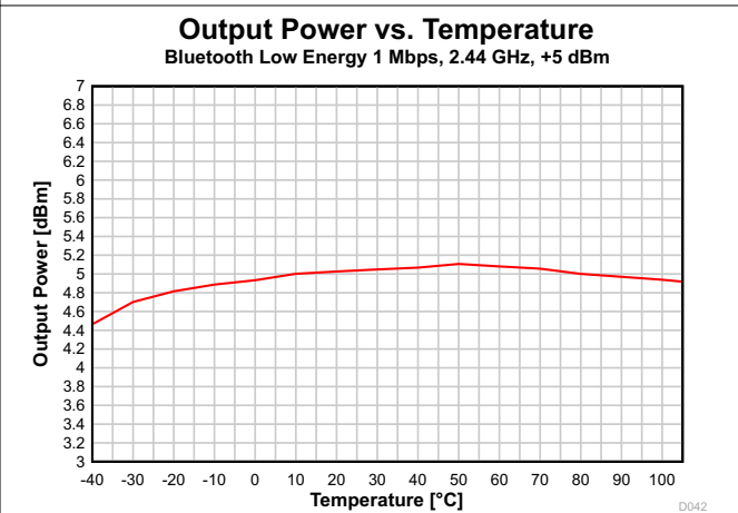
图 7-38. Output Power vs. Temperature (Bluetooth Low Energy 1 Mbps, 2.44 GHz, +5 dBm)
