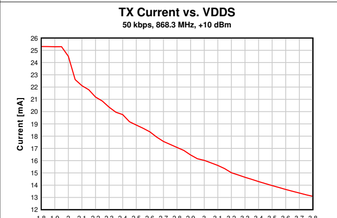
图 7-15. TX Current vs. Supply Voltage (VDD5) (50 kbps, 868.3 MHz)
