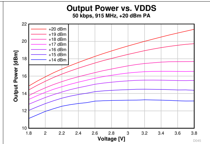
图 7-42. Output Power vs. Supply Voltage (VDD5) (50 kbps, 915 MHz)
