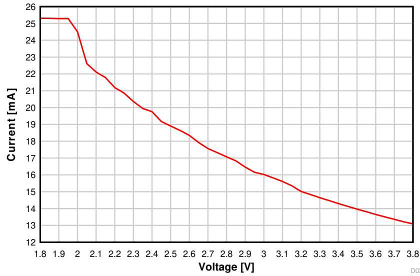
图 8-18. TX Current vs. Supply Voltage (VDDS) (50 kbps, 868.3 MHz)
