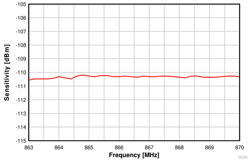
图 8-23. Sensitivity vs. Frequency (50 kbps, 868 MHz)
