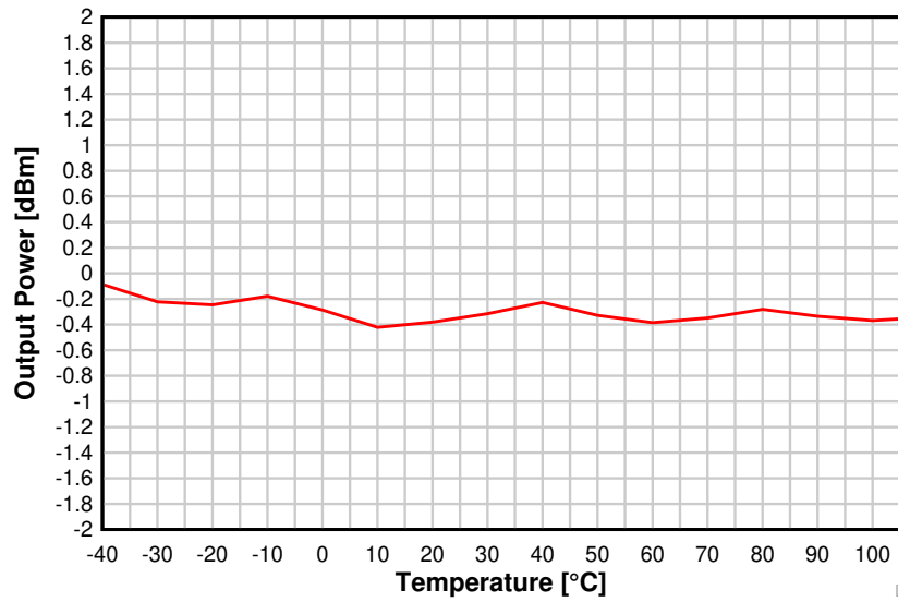
图 8-41. Output Power vs. Temperature (BLE 1 Mbps, 2.44 GHz)
