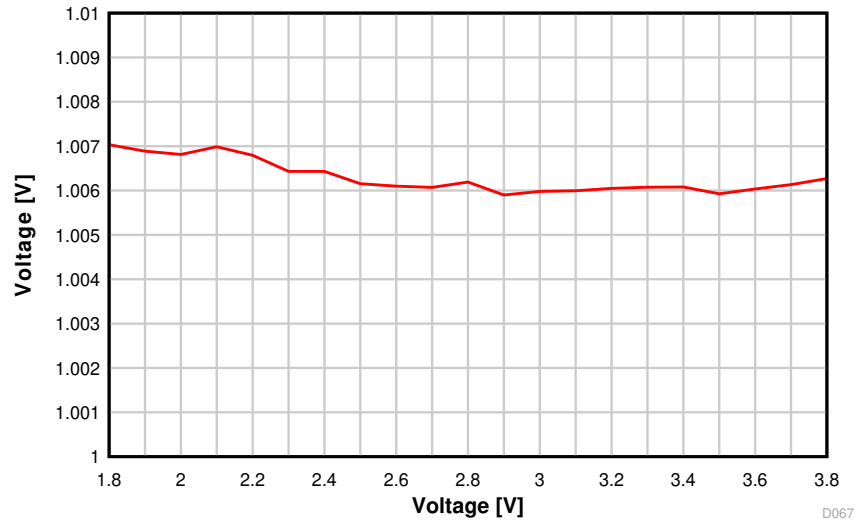
图 8-63. ADC Accuracy vs. Supply Voltage (VDDS)
