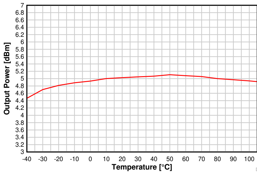
图 8-42. Output Power vs. Temperature (BLE 1 Mbps, 2.44 GHz, +5 dBm)
