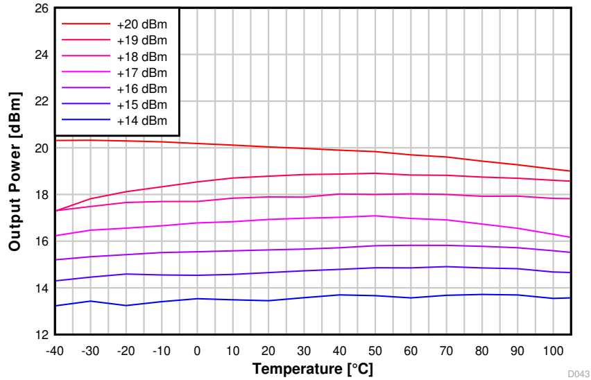
图 8-43. Output Power vs. Temperature (BLE 1 Mbps, 2.44 GHz, +20 dBm PA)
