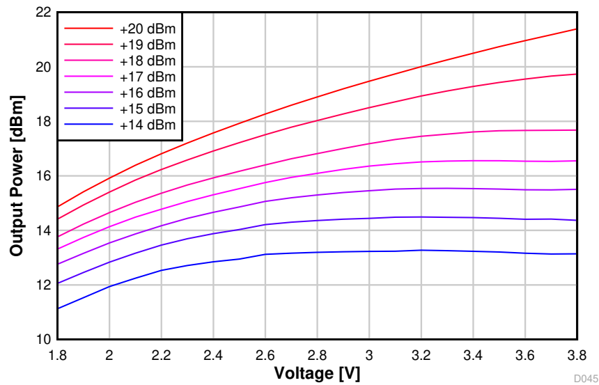
图 8-46. Output Power vs. Supply Voltage (VDD5) (50 kbps, 915 MHz)
