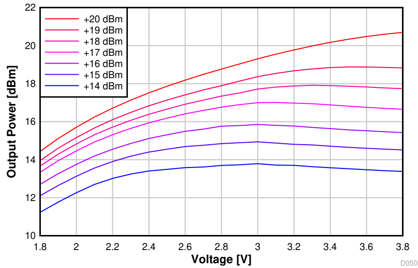
图 8-49. Output Power vs. Supply Voltage (VDDS) (BLE 1 Mbps, 2.44 GHz, +20 dBm PA)
