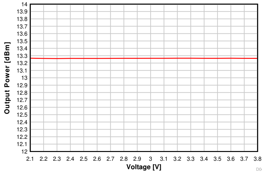
图 8-45. Output Power vs. Supply Voltage (VDD5) (50 kbps, 868.3 MHz)
