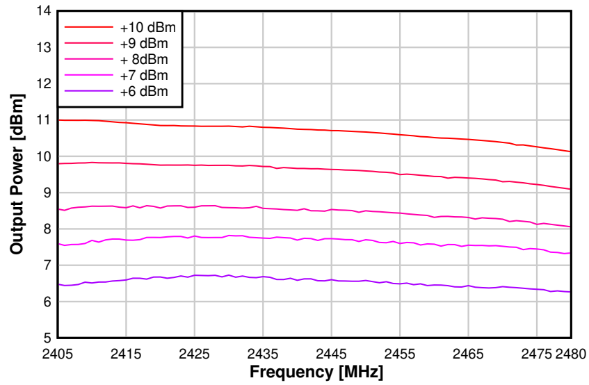
图 8-57. Output Power vs. Frequency (250 kbps, +10 dBm PA)
