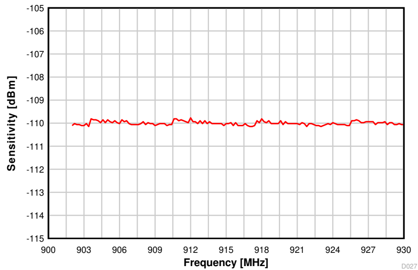
图 8-24. Sensitivity vs. Frequency (50 kbps, 915 MHz)
