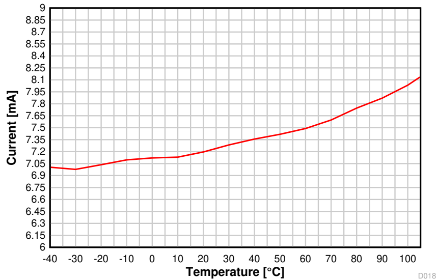
图 8-15. TX Current vs. Temperature (BLE 1 Mbps, 2.44 GHz)
