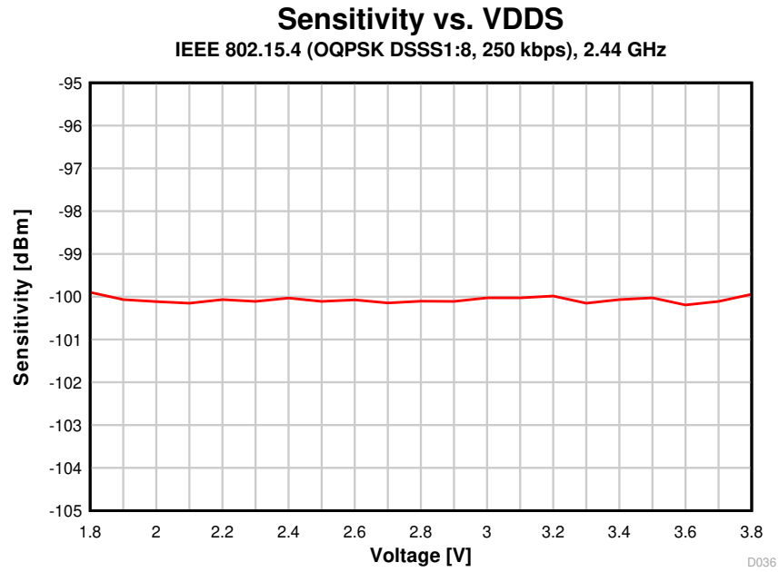
8-33. Sensitivity vs. Supply Voltage (VDDS) (250 kbps, 2.44 GHz)
