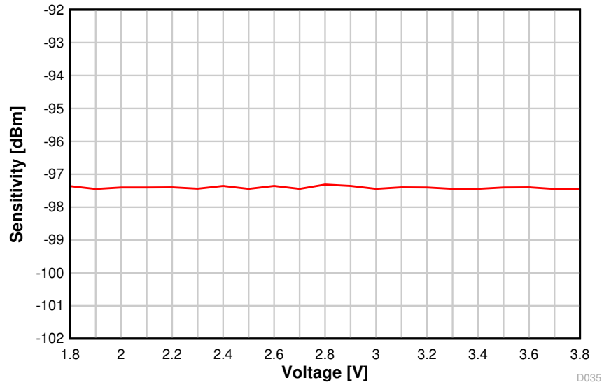
图 8-32. Sensitivity vs. Supply Voltage (VDDS) (BLE 1 Mbps, 2.44 GHz, DCDC Off)
