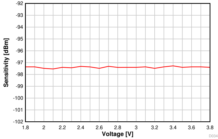
图 8-31. Sensitivity vs. Supply Voltage (VDDS) (BLE 1 Mbps, 2.44 GHz)
