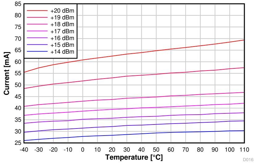
图 8-14. TX Current vs. Temperature (50 kbps, 915 MHz, VDDS = 3.3 V)
