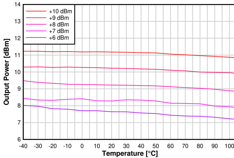
图 8-44. Output Power vs. Temperature (2.44 GHz, +10 dBm PA)
