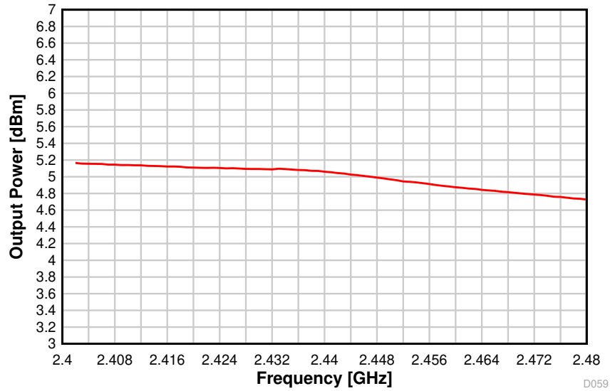
图 8-55. Output Power vs. Frequency (BLE 1 Mbps, 2.44 GHz, +5 dBm)
