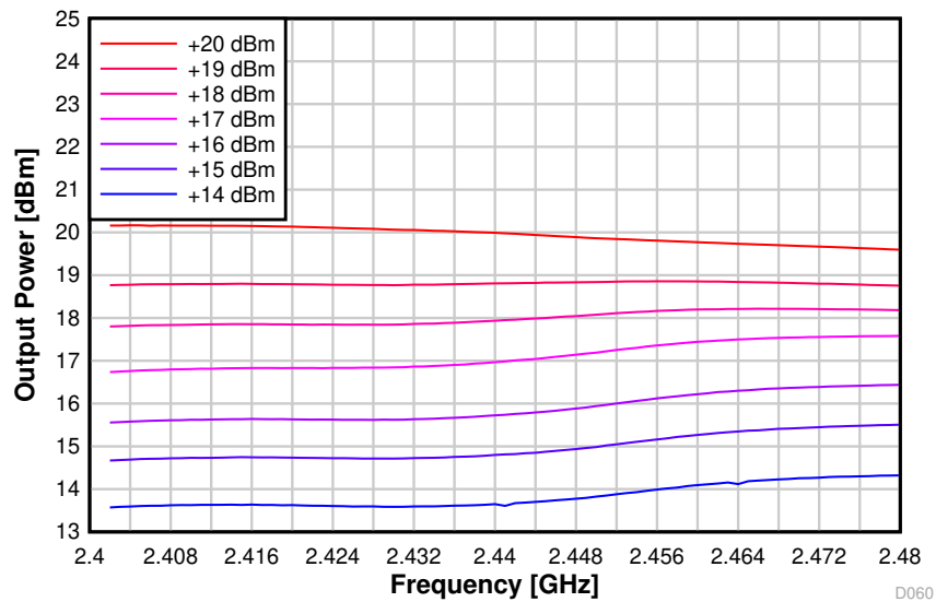
图 8-56. Output Power vs. Frequency (BLE 1 Mbps, 2.44 GHz, +20 dBm PA)
