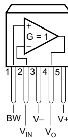
图 5-3. KTT Package, 5-Pin TO-263 (Top View)
