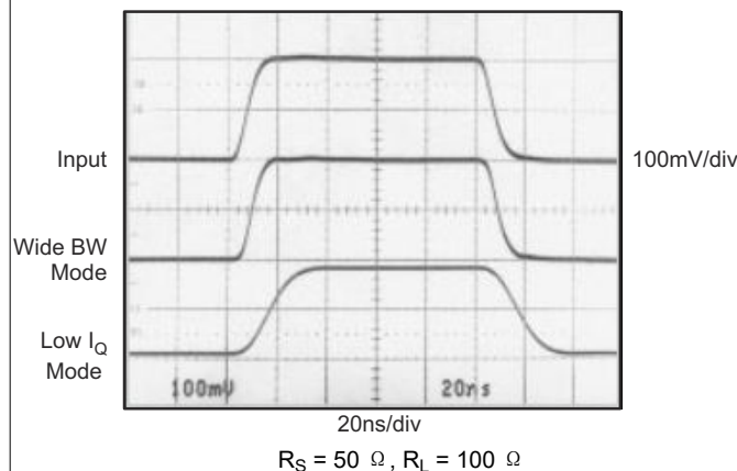
图 6-17. Small-Signal Response
