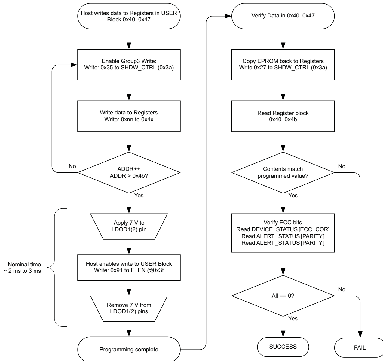
Figure 15. EPROM Programming
