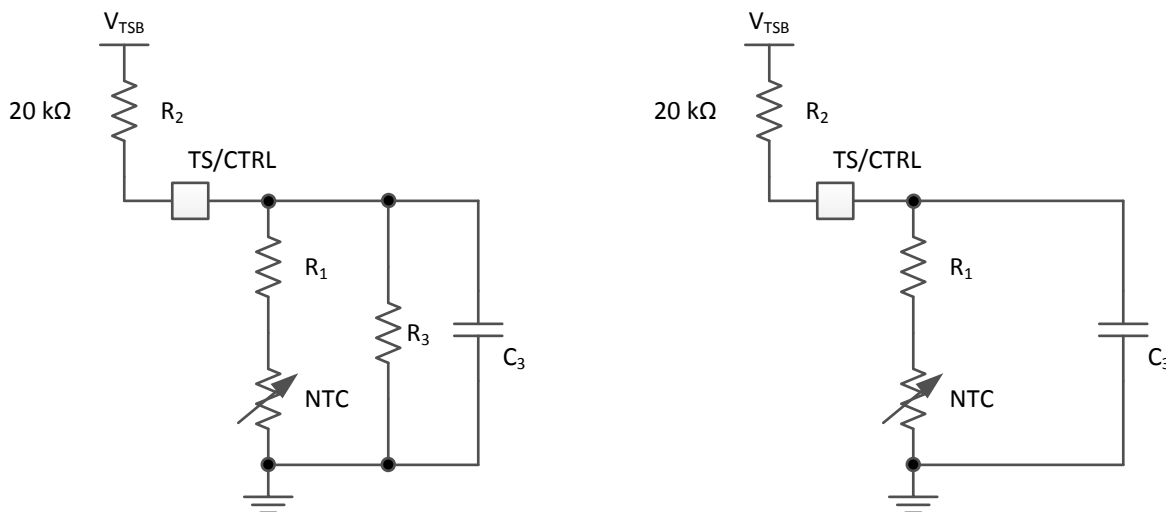
图 8-12. NTC Circuit Options For Safe Operation of the Wireless Receiver Power Supply
