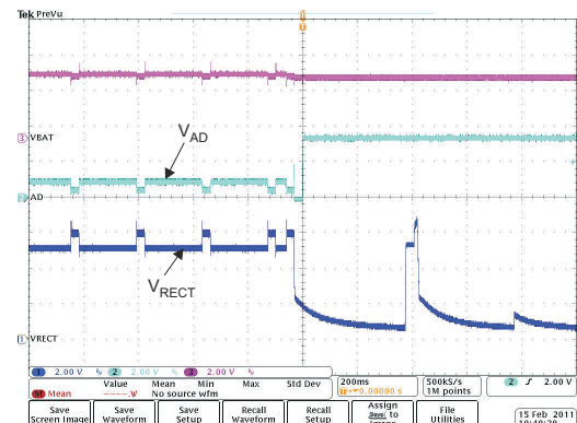
图 7-16. On-the-Go Enabled ( V_{OTG} = 3.5 \text{ V} ) (3)
