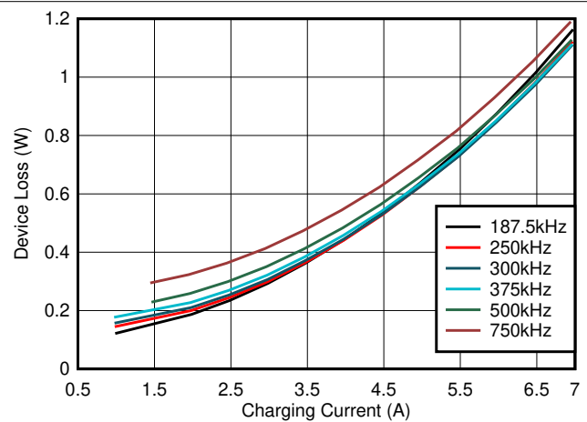
图 8-4. BQ25968 Device Power Loss, 4 x 22-μF Caps Per Phase
