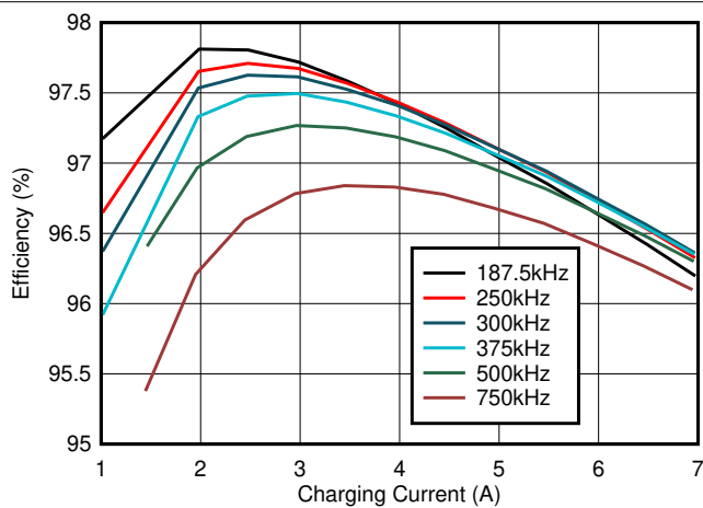
图 8-3. BQ25968 Device Efficiency, 4 x 22-μF Caps Per Phase
