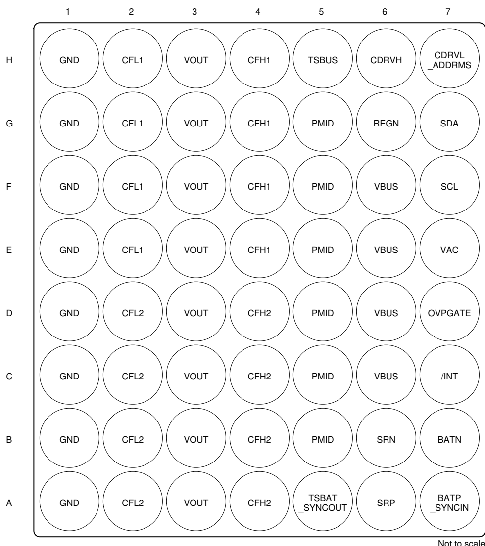
图 7-1. YFF Package 56-Pin DSBGA Bottom View
