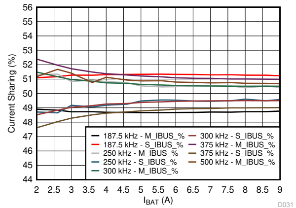
图 8-6. BQ25968 Parallel Current Sharing
