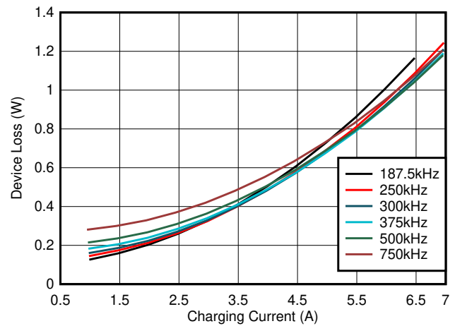
图 8-2. BQ25968 Device Power Loss, 4 x 20-μF Caps Per Phase
