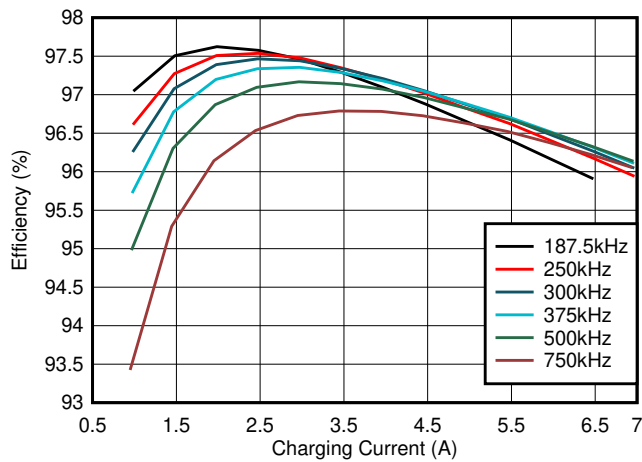
图 8-1. BQ25968 Device Efficiency, 3 x 22-μF Caps Per Phase
