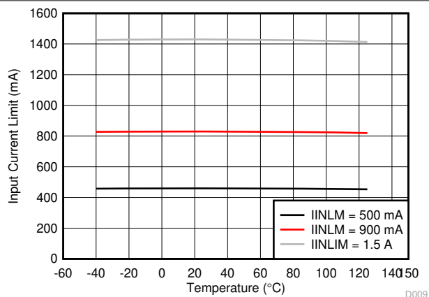
图 8-8. Input Current Limit vs Temperature
