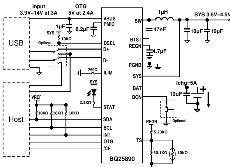
图 10-1. BQ25890 with D+/D- Interface and USB On-The-Go (OTG)
