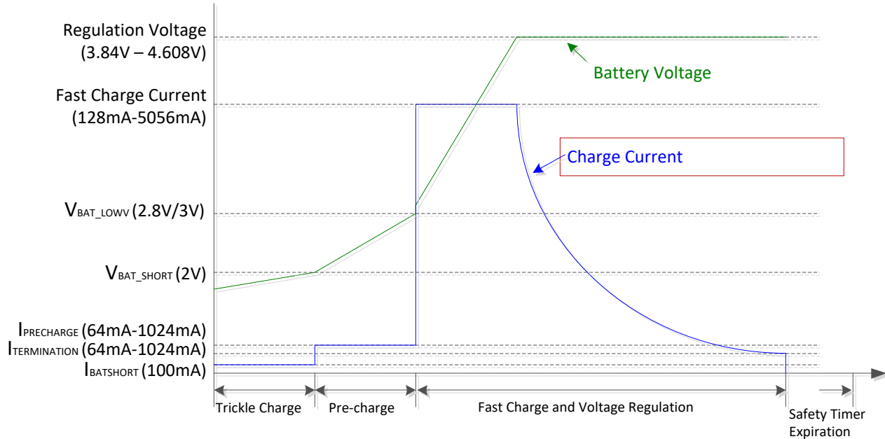
图 9-5. Battery Charging Profile
