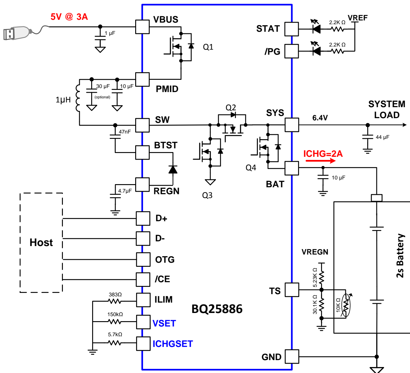
图 20. BQ25886 (Stand-Alone) Typical Application Diagram
