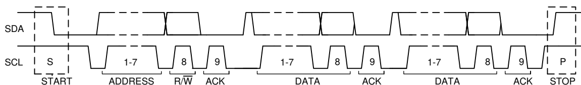
图 9-20. Complete Data Transfer on the I 2 C Bus
