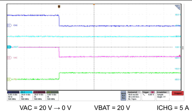
图 9-4. VAC Un-plug Power Down with 5-A ICHG
