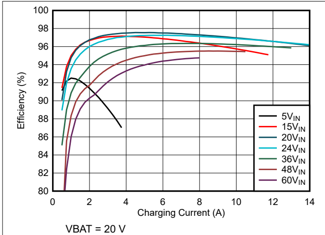
图 7-1. Charge Efficiency vs Charge Current (5s battery configuration)
