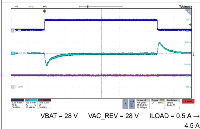
图 9-17. Reverse Mode Buck-Boost Transient Reponse
