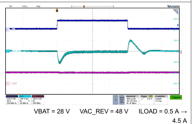
图 9-18. Reverse Mode Boost Transient Reponse
