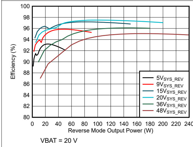
VBAT = 20 V 图 7-9. Reverse Mode Efficiency (5s battery configuration)
