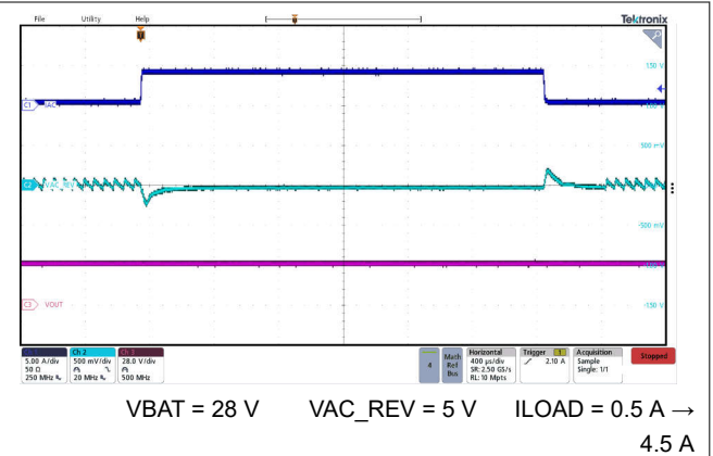
图 9-16. Reverse Mode Buck Transient Reponse
