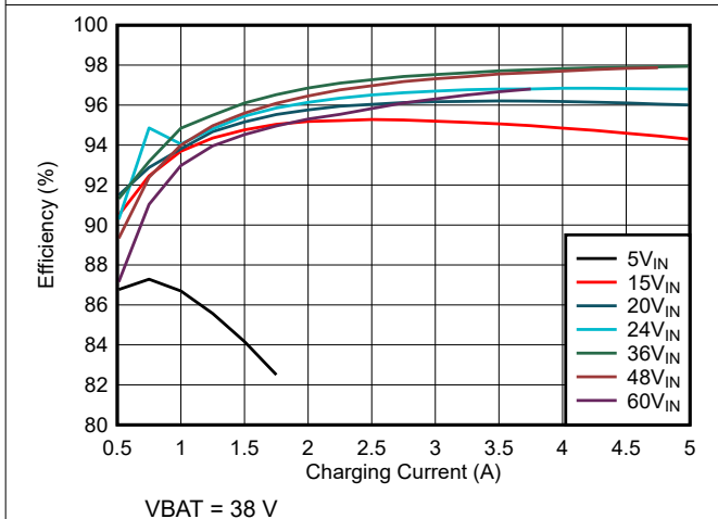
图 7-3. Charge Efficiency vs Charge Current (10s battery configuration)
