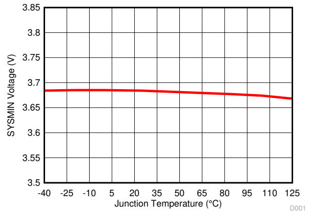
图 8-4. SYSMIN Voltage vs. Junction Temperature
