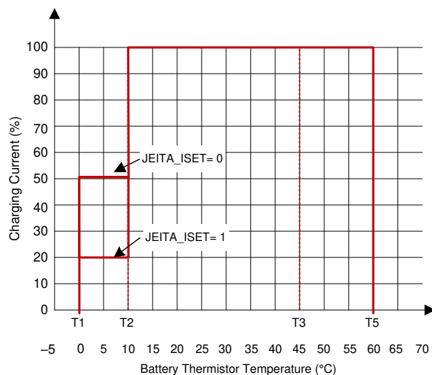
图 9-3. JEITA Profile: Charging Current
