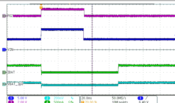
图 8-5. Charge Disable
