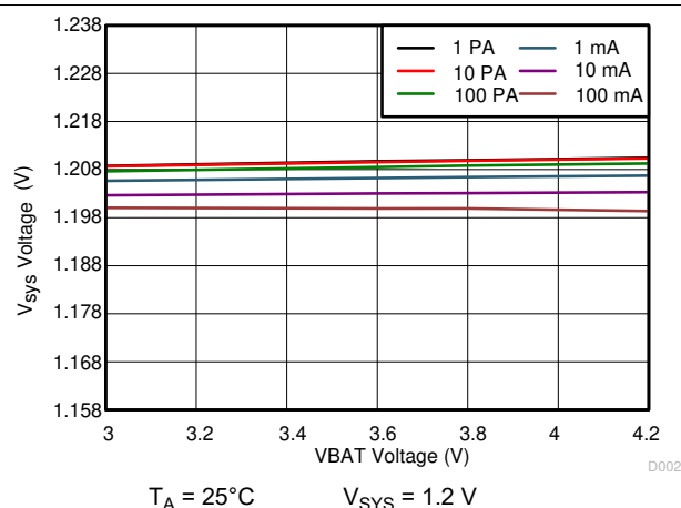
图 10-18. 1.2 V_{\text{SYS}} Line Regulation
