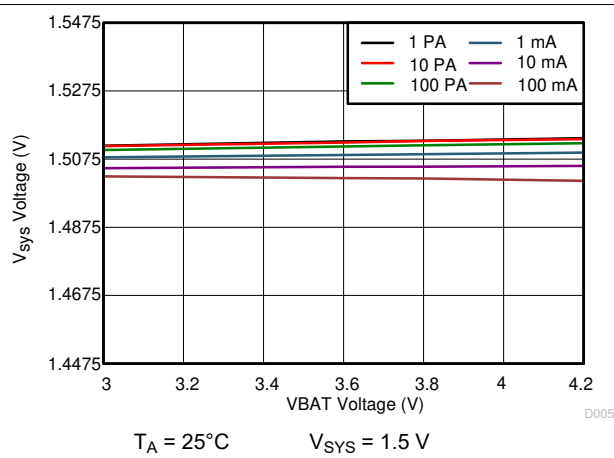
图 10-19. 1.5 V_{\text{SYS}} Line Regulation
