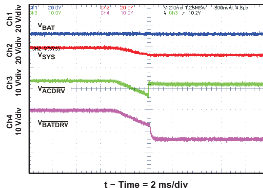
Figure 20. System Selector On Adapter Removal With 390 \mu F SYS-to-PGND System Capacitor
