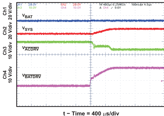
Figure 19. System Selector On Adapter Insertion With 390 \mu F SYS-to-PGND System Capacitor
