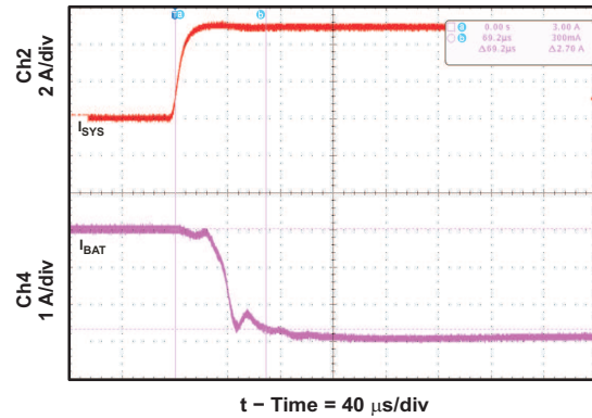
Figure 13. Fast DPM Response
