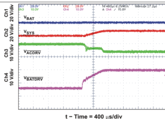
Figure 20. System Selector On Adapter Removal With 390 \mu F SYS-to-PGND System Capacitor
