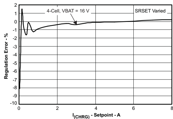
Figure 8. Charge Current Regulation Accuracy
