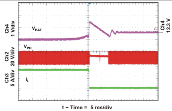
Figure 16. Battery Removal
