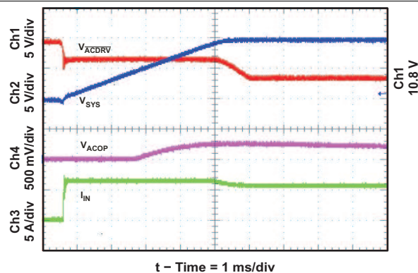
Figure 22. System Selector Learn Turnoff With 390 \mu F SYS-to-PGND System Capacitor
