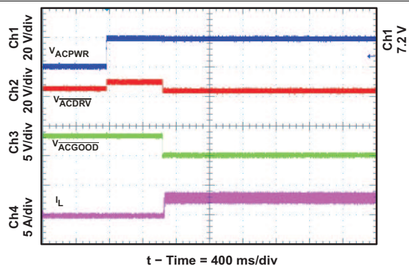
Figure 21. System Selector Learn Turnon With 390 \mu F SYS-to-PGND System Capacitor
