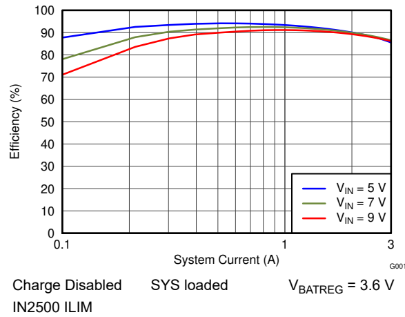
图 7-1. IN Efficiency
