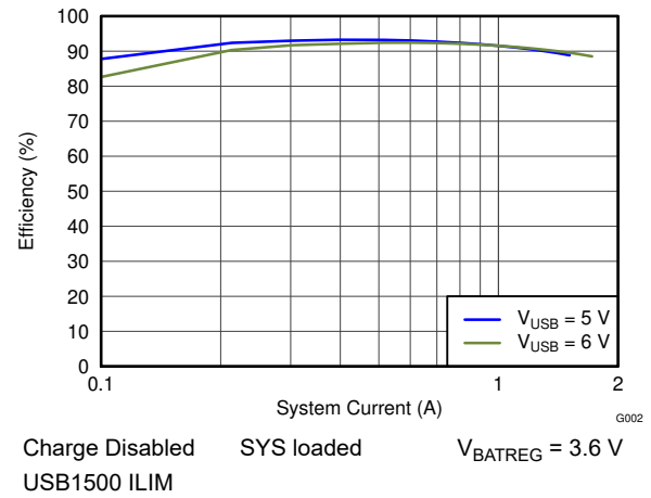
图 7-2. USB Efficiency
