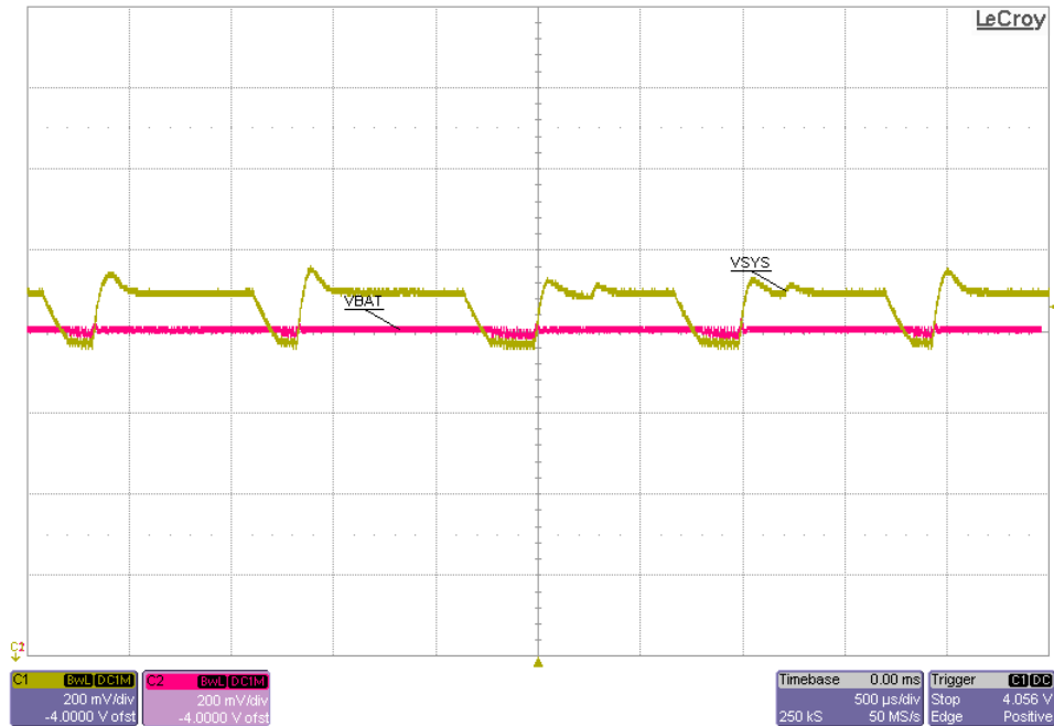
Figure 25. Reverse Boost
