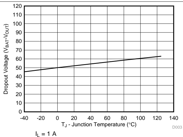
图 16. Dropout Voltage vs Temperature
