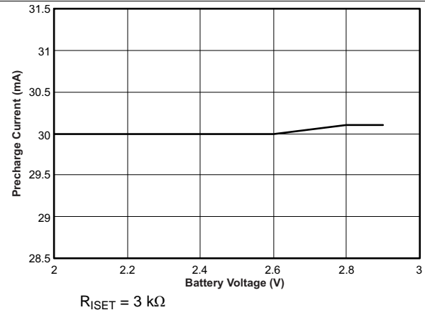
图 13. Precharge Current vs Battery Voltage
