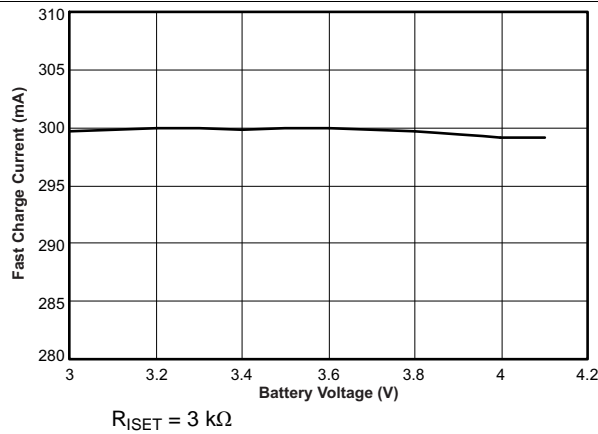
图 12. Fastcharge Current vs Battery Voltage
