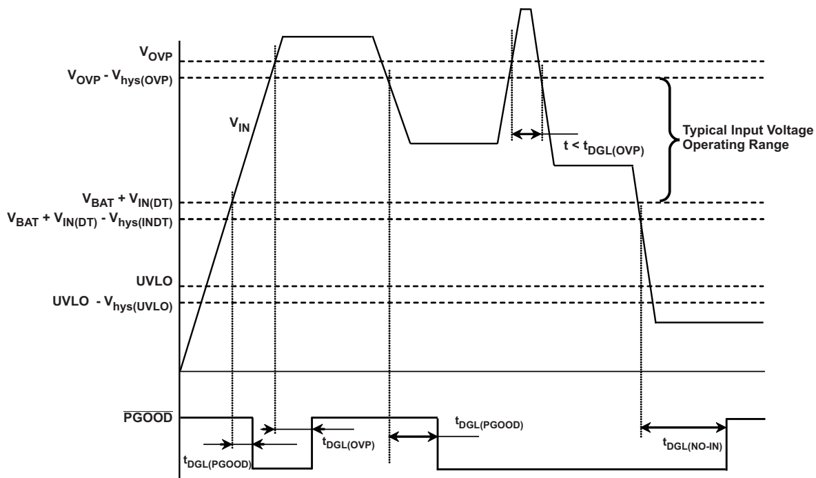
图 1. Power-Up, Power-Down, Power Good Indication
