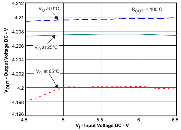
图 2. Line Regulation
