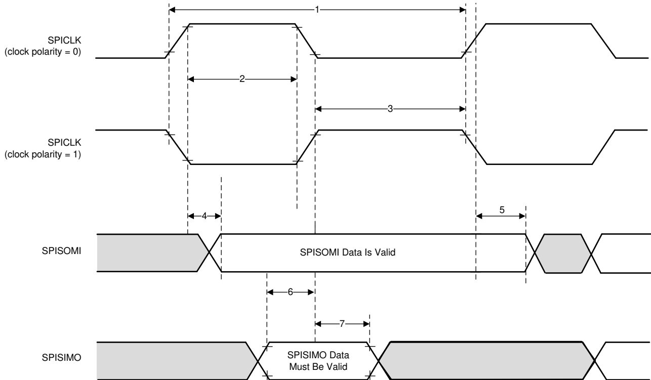
图 8-10. SPI Peripheral Mode External Timing (CLOCK PHASE = 0)
