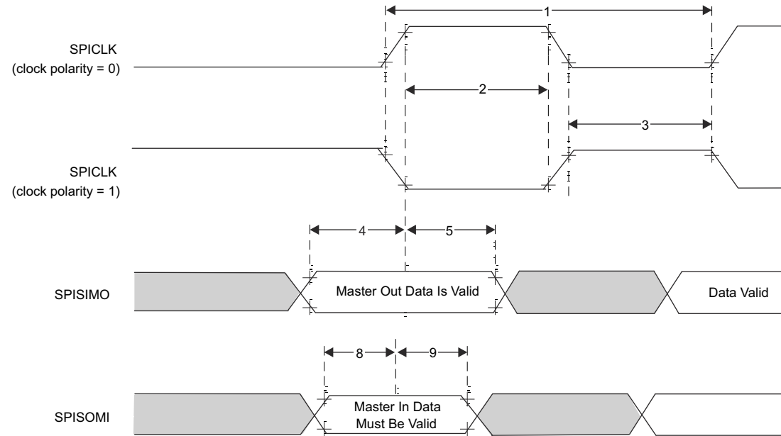
图 8-8. SPI Controller Mode External Timing (CLOCK PHASE = 1)
