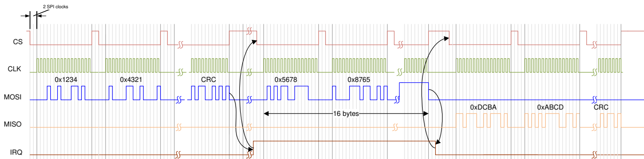
图 8-12. SPI Communication
