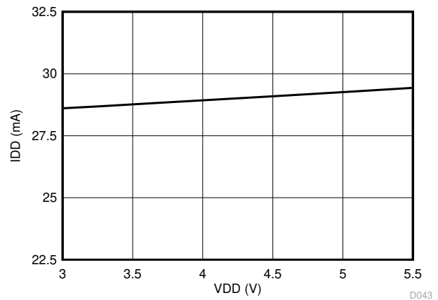
图 5-34. Input-Supply Current vs Supply Voltage
