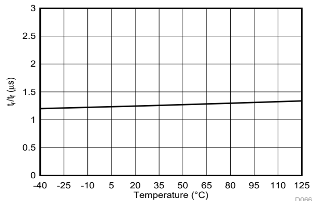
图 6-41. Output Rise and Fall Time vs Temperature
