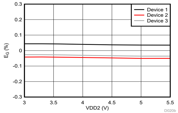
图 6-12. Gain Error vs Low-Side Supply Voltage
