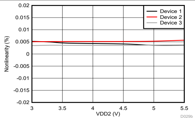
图 6-16. Nonlinearity vs Low-Side Supply Voltage
