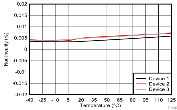
图 6-17. Nonlinearity vs Temperature
