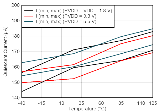
图 6-51. PVDD Supply Current vs Temperature
