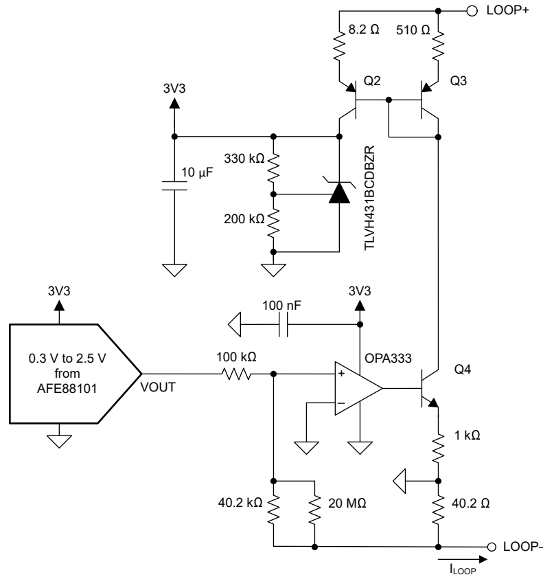
图 8-5. Current Loop Control for the AFE88101 Transmitter
