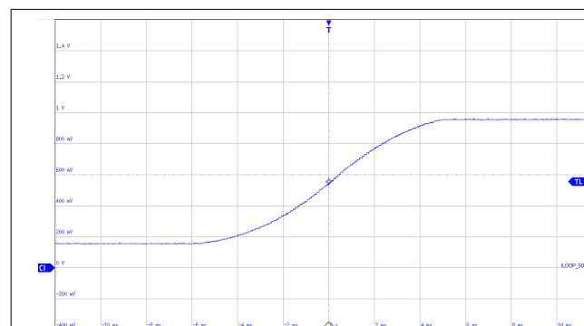
图 7-5. Sinusoidal Slew Rate: Rising
