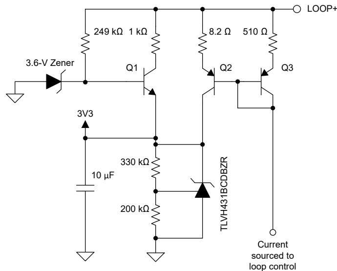
图 8-4. Start-Up Circuit
