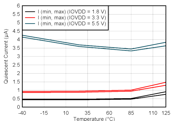
图 6-52. IOVDD Supply Current vs Temperature
