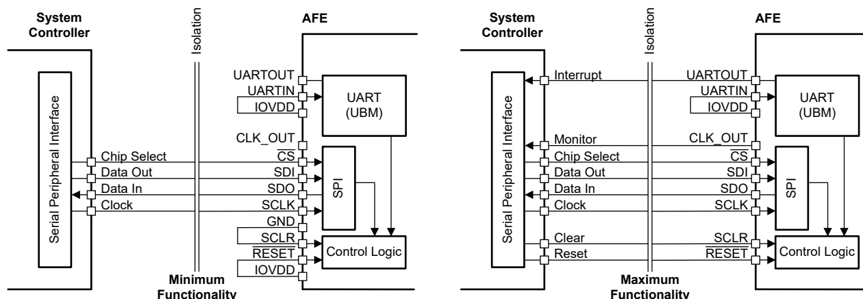
图 7-17. SPI Mode Connections
