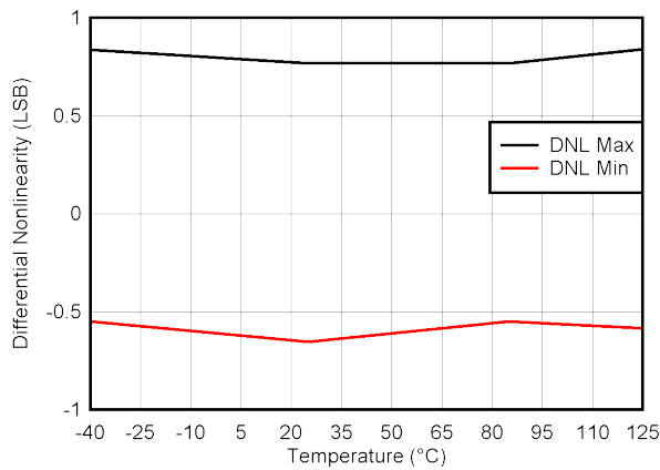
图 6-37. ADC DNL Range vs Temperature
