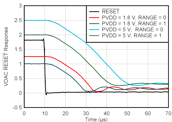
图 6-12. DAC RESET Response
