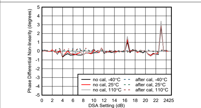
图 4-427. RX Phase Differential Nonlinearity at 8.11GHz
