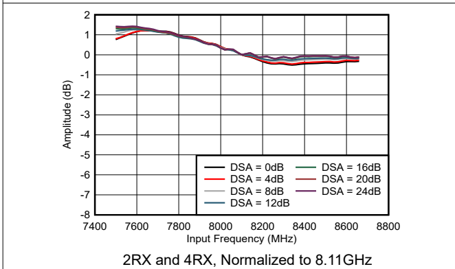
图 4-424. RX Amplitude vs Frequency and DSA Setting
