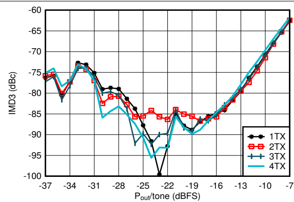
图 4-28. TX IMD3 vs Digital Level at 0.85GHz
