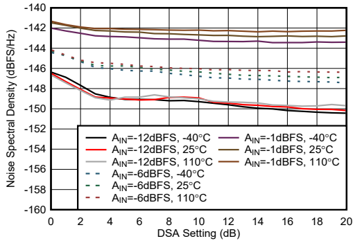
图 4-461. RX NSD vs DSA Setting at 9.6GHz
