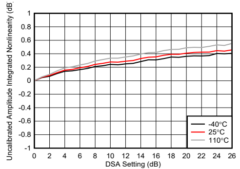
图 4-242. TX DSA Uncalibrated Amplitude Integrated Nonlinearity
