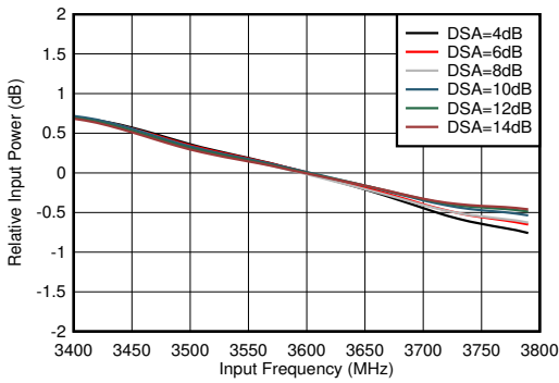
图 4-366. RX In-Band Gain Flatness, f_{IN} = 3600\text{MHz}
