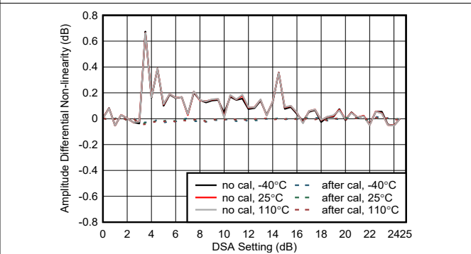
图 4-425. RX Amplitude Differential Nonlinearity at 8.11GHz
