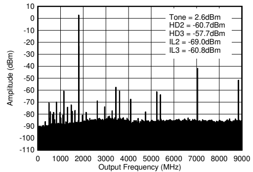
图 4-75. TX Single Tone (-12 dBFS) Output Spectrum at 1.8GHz ( 0-f_{\text{DAC}} )
