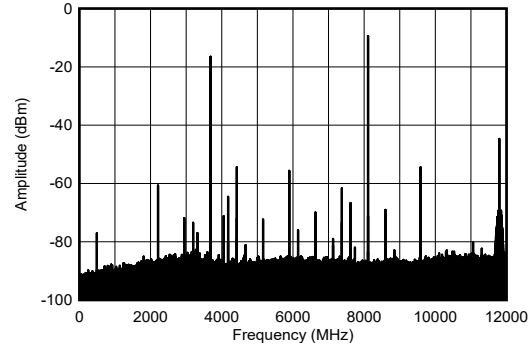
-6dBFS 图 4-205. TX Single Tone Output Spectrum at 8.1GHz
