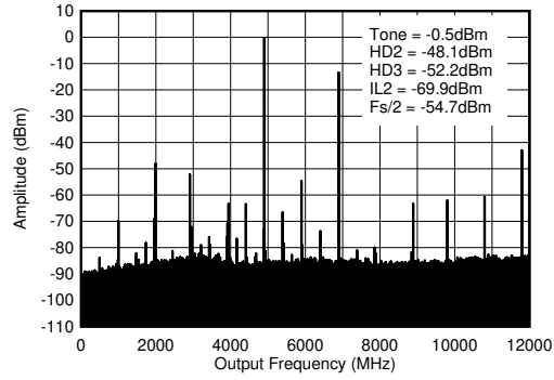
图 4-183. TX Single Tone (-1 dBFS) Output Spectrum at 4.9GHz (0- f_{\text{DAC}} )
