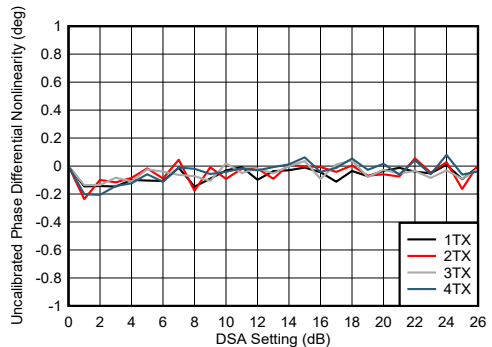
图 4-244. TX DSA Uncalibrated Phase Differential Nonlinearity
