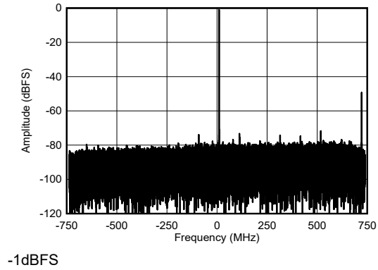
图 4-466. RX Single Tone Output FFT at 9.61 GHz
