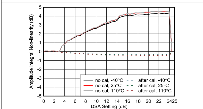
图 4-426. RX Amplitude Integrated Nonlinearity at 8.11GHz
