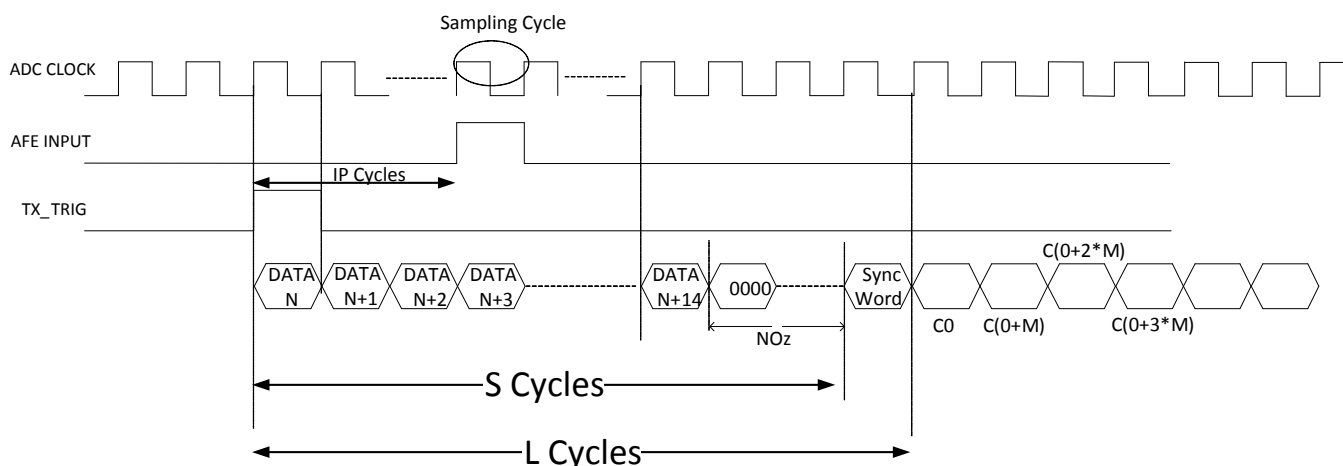
Figure 74. Measured Latency Timing at any M
