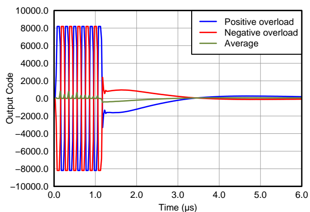
Figure 56. Pulse Inversion, V_N = 2 Vpp, PRF = 1 KHz, Gain = 21 dB
