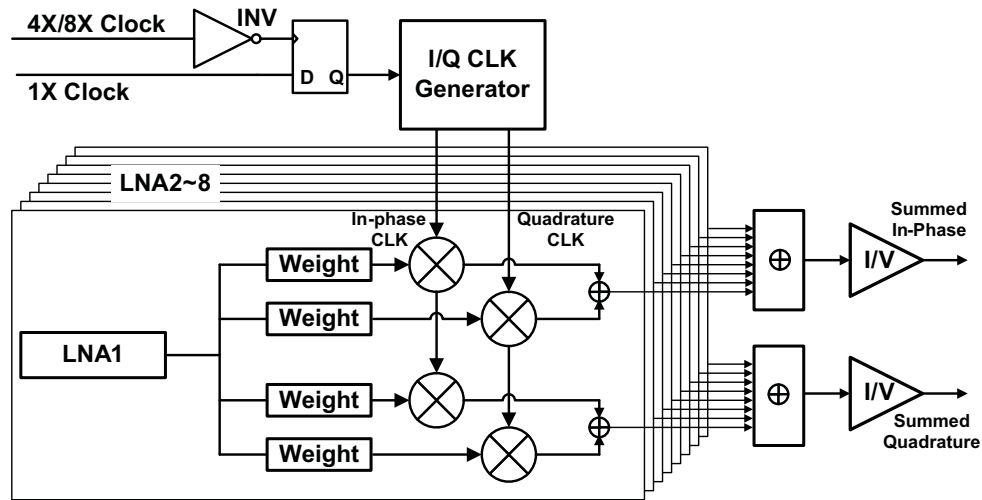
Figure 73. 8 X f cw and 4 X f cw Block Diagram
