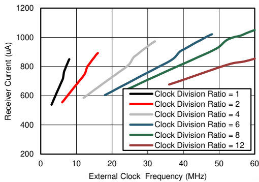
图 7-7. Receiver Currents (Analog and Digital) vs Clock Divider Ratio
