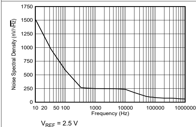
图 6-16. DAC Noise Voltage vs Frequency
