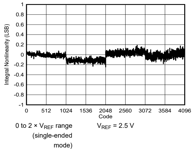
图 6-23. Integral Linearity Error vs Code
