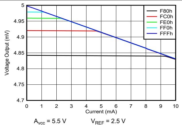
图 6-13. Output Voltage vs Source Current Capability
