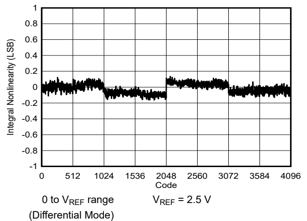
图 6-25. Integral Linearity Error vs Code
