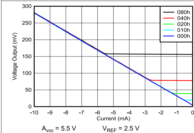
图 6-14. Output Voltage vs Sink Current Capability
