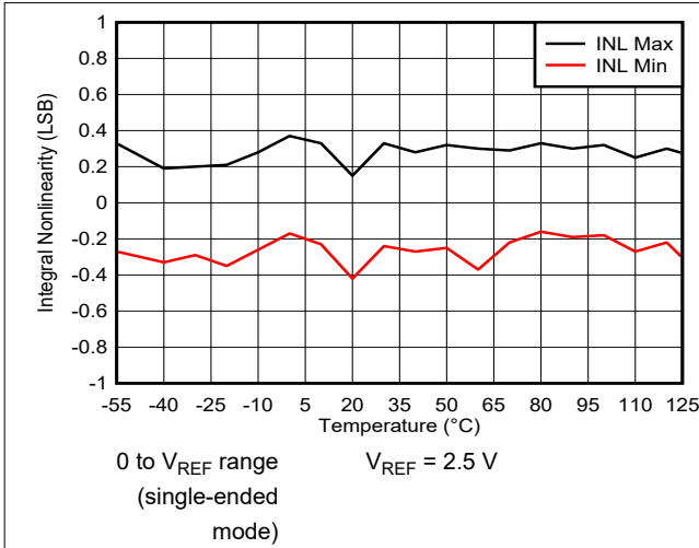
图 6-32. Integral Linearity Error vs Temperature
