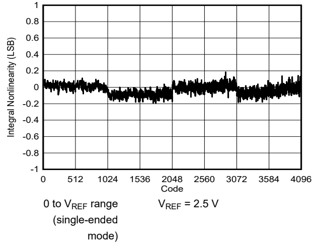
图 6-21. Integral Linearity Error vs Code
