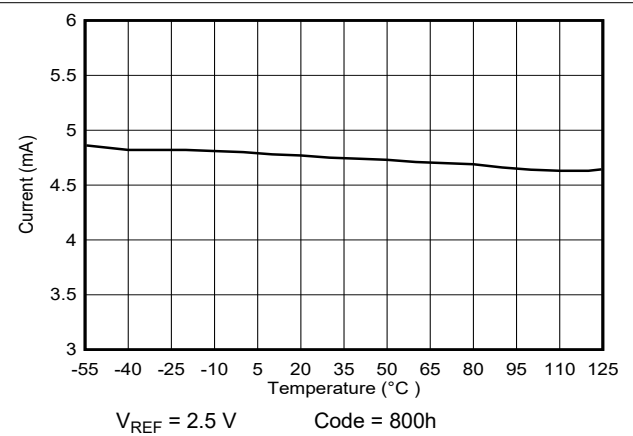
图 6-15. Supply Current vs Temperature
