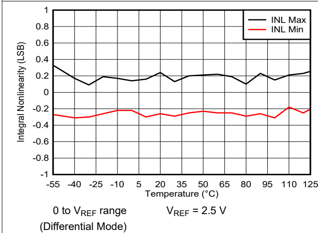
图 6-34. Integral Linearity Error vs Temperature
