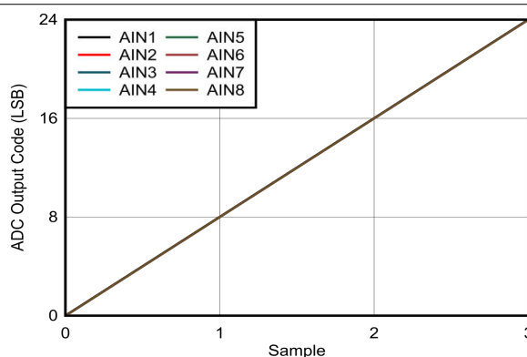
图 7-39. 斜坡测试图形示例，阶跃 = 8 ( TP_AIN1 = 7、TP_UPD_MODE = 1 )
