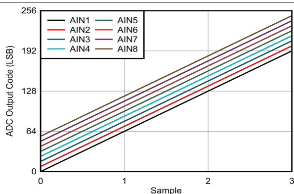
图 7-38. 斜坡测试图形示例，阶跃 = 8 ( TP_AIN1 = 7、TP_UPD_MODE = 0 )
